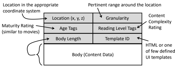
Figure 2: An application level protocol to enable unidirectional broadcast information flow that contains sufficient information for rendering content on the mobile application.
