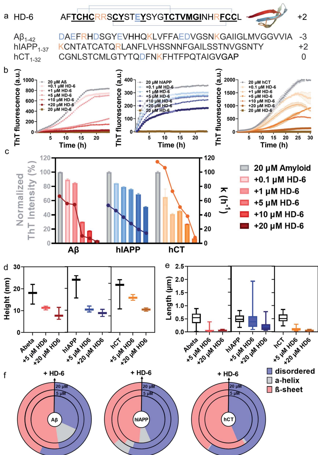
Fig. 1 HD-6 exhibits a general cross-seeding-induced inhibition capacity against different amyloid aggregation pathways. (a) Sequence and structure of HD-6, Ab, hIAPP, and hCT with b-rich structure. Color ID: positively charged residues (orange letters), negatively charged residues (blue letters), and b-structure fragments (bold & underline). (b) ThT aggregation kinetic profiles and (c) quantitative analysis of ThT profiles to show the dose-dependent inhibition effects of HD-6 on Ab, hIAPP, and hCT aggregation at different amyloid : HD-6 ratios (1 : 0.005–1 : 1). Inhibition efficiency of HD-6 against amyloid aggregation is determined by the relative final fluorescence intensity (%) as normalized by that of pure amyloid aggregation (left axis). Error bar represents the standard deviation (s.d.) of triplicate measurements. The corresponding aggregation rate constant ( k ) is determined by a time point of t_{1/2} , at which the fluorescence intensity reaches half of the maximum fluorescence intensity.
