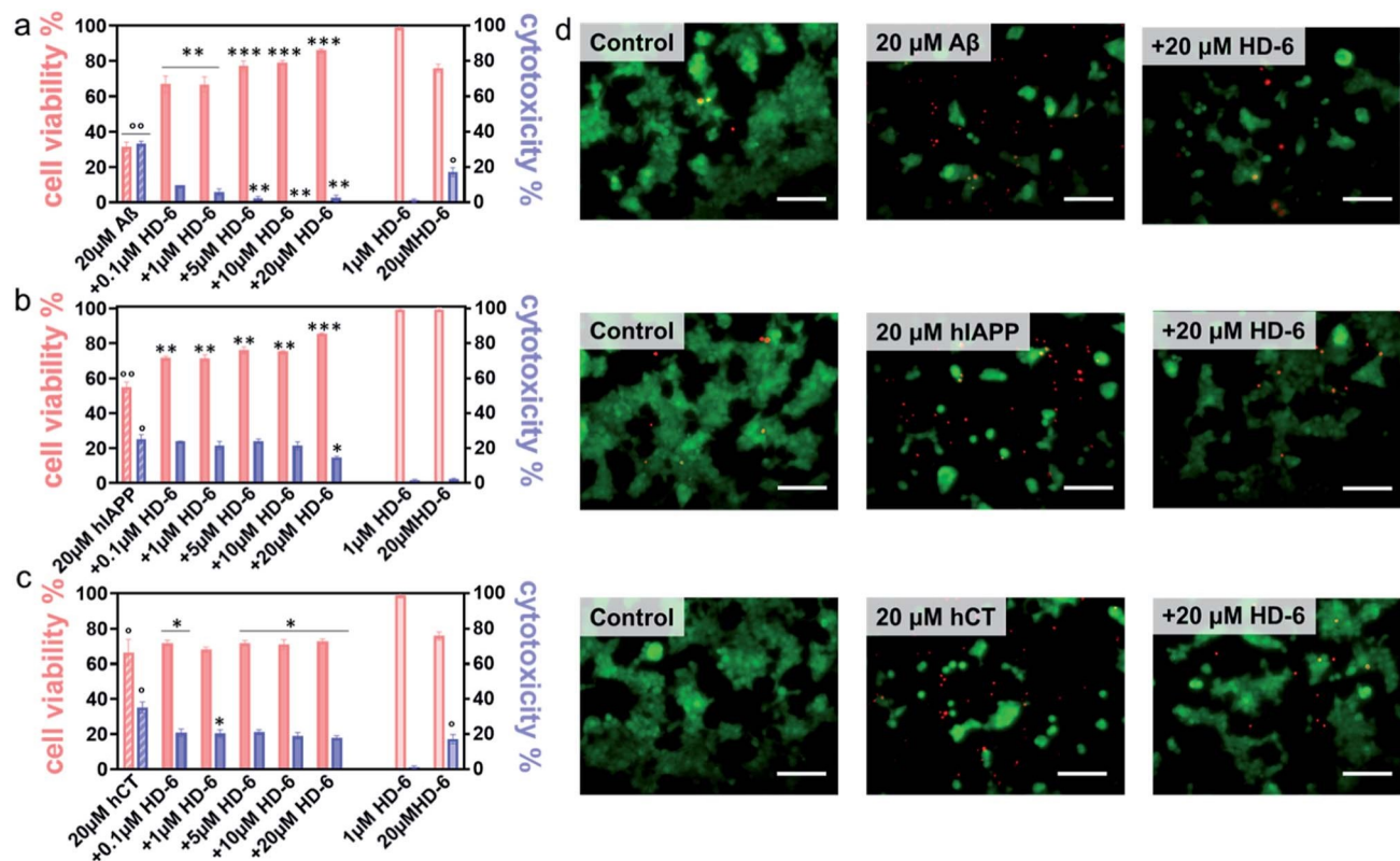
Fig. 4 HD-6 rescues cells from amyloid-induced cytotoxicity. Dose-dependent protection role of HD-6 in (a) Ab-, (b) hIAPP-, and (c) hCT-mediated cytotoxicity using cell viability from the MTT assay (red bar, left axis) and cell cytotoxicity from the LDH assay (blue bar, right axis), in which SH-SY5Y cells or RIN-m5F cells are treated with amyloid (20 mM) with and without 0.1–20 mM HD-6 for 24 h. Statistical analysis ( n \geq 3 ) was conducted for cells treated with HD-6 or amyloid proteins alone relative to control ( p < 0.05 ; p < 0.01 ; p < 0.001 ), as well as cells treated with both HD-6 and amyloid proteins relative to cells treated with amyloid proteins alone (*, p < 0.05 ; **, p < 0.01 ; ***, p < 0.001 ). (d) Representative fluorescence microscopy images of cells upon treatment with 20 mM HD-6 (1 st column), 20 mM amyloid proteins (2 nd column), and their cross-seeds (3 rd column) for 24 h. Scale bars \frac{1}{4} 180 \mu m.
