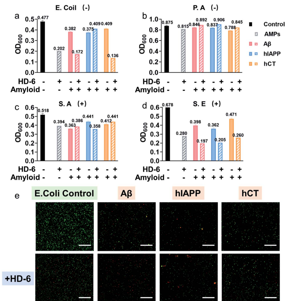
Fig. 5 HD-6–amyloid heterocomplex retains a broad-spectrum antimicrobial activity. Antimicrobial activity of 20 mM HD-6, 20 mM amyloid peptides, and cross-species of HD-6–amyloid peptides against Gram-negative (a) E. coli and (b) P. aeruginosa , and Gram-positive (c) S. aureus and (d) S. epidermidis quantified by the final bacterial density. Bacterial density is determined by OD 600 . (e) Representative fluorescence microscopy images of E. coli treated with freshly prepared amyloid peptides (20 mM) in the absence and presence of 20 mM HD-6. Red fluorescent propidium iodide and green fluorescent SYTO 9 are used to identify dead bacteria with damaged membranes and live bacteria with intact membranes, respectively. Scale bars \frac{1}{4} 180 nm.
