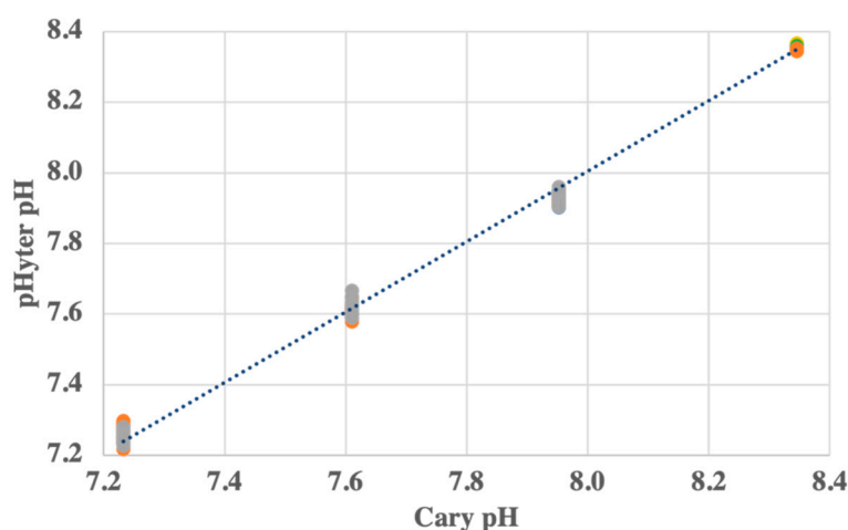
Figure 3. (pHyter versus Cary seawater pH measurements). Seawater pH measurements made by pHyters in relation to Cary UV-Vis measurements at four pH values between 7.2 and 8.3. The slope of the linear fit is 0.997, R^2 = 0.998 , n = 69 ). Six pHyters were used, shown in yellow, turquoise, green, blue, orange, and gray.
