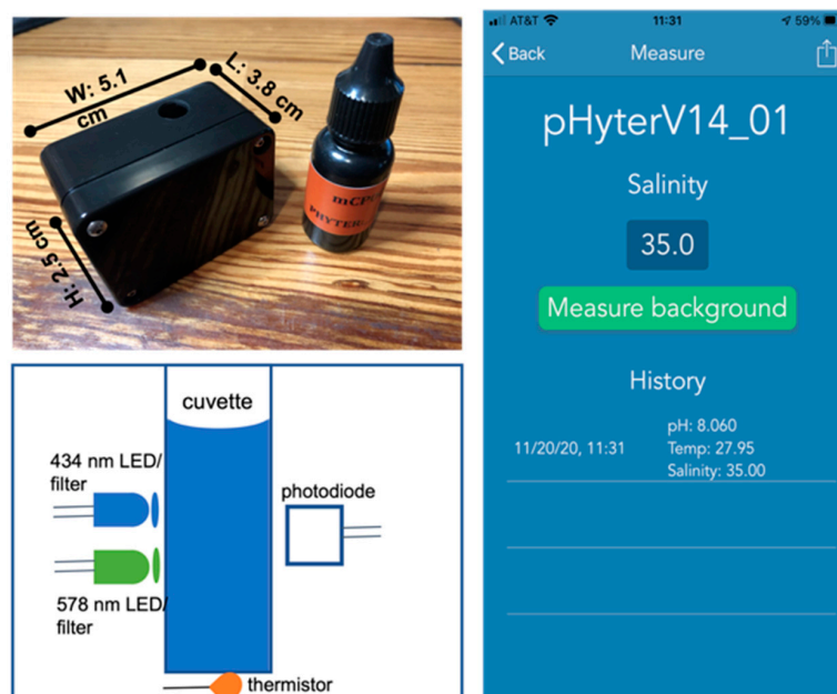
Figure 1. (The pHyer). The pHyer next to an mCP reagent bottle ( upper left ); pHyer optical design ( lower left ); and pHyer phone app ( right ).
