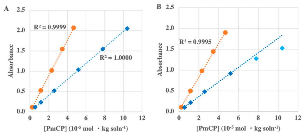
Figure 2. (Absorbance linearity). Absorbance was measured in triplicate by the pHHyter over a range of mCP concentrations at pH 5 and 11. The orange circles represent 578 nm absorbance from the pH 11 solution; the blue diamonds represent 434 nm absorbance from the pH 5 solution. The light blue diamonds represent points deviating from the linear response at 434 nm. (A) A pHHyter with 10-nm bandpass filters on each LED; (B) a pHHyter without bandpass filters.
