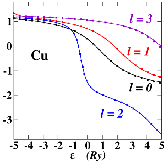
FIG. 11. Plot of all-electron A_l(\varepsilon) (full lines) and pseudo \tilde{A}_l(\varepsilon) (enlarged dots) plotted in units of radians along the vertical axis for a Cu atom calculated using r2SCAN with \eta = 0.01 for the angular momentum channels l = 0, 1, 2 , and 3 for the indicated energy range. In this case, the core states were taken to be 1s^2 2s^2 2p^6 , the valence configuration was 3s^2 3p^6 3d^{10} 4s^1 4p^0 , and the augmentation radius was r_c^a = 1.8 Bohr. The basis set included two basis functions for each l channel for l = 0, 1, 2 , including a continuum state for l = 2 .
