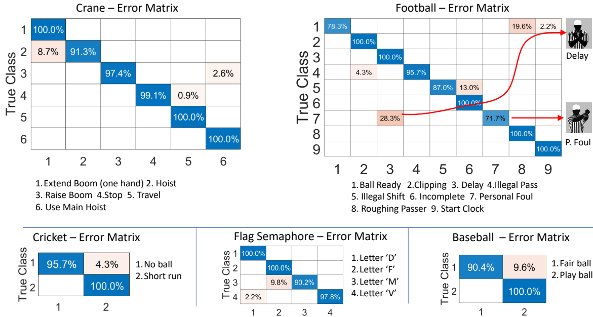
Fig. 16. Confusion matrices for five different applications. Only error confusions plotted for each application. Confusion occurs between very similar actions, as illustrated in the football case.
