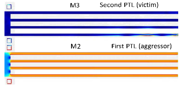
Fig. 5. Current distribution within coupled stripline with the four narrow line topology operating at around 20 GHz.
