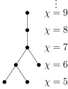
FIGURE 4. An example of a graded root.
