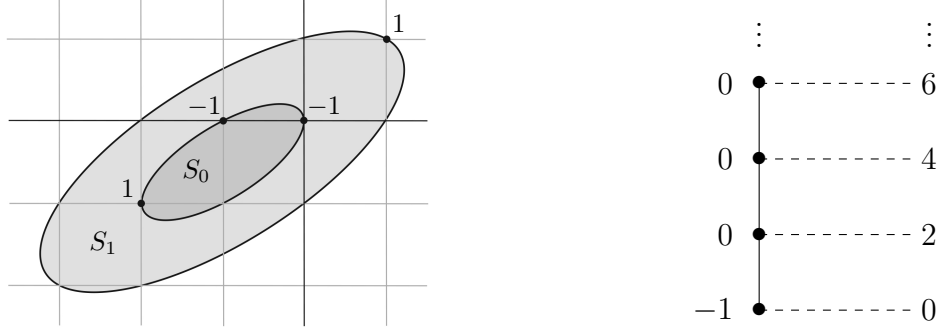
FIGURE 5. Left: the sublevel sets S_0 and S_1 from Example 4.5. The four contributing lattice points and their F_{\Gamma,k} -weights are indicated. Right: the corresponding graded root, with the weights from Equation (12) written to the left of each vertex. Recall from grading conventions 3.5 that the numbers 0, 2, 4, 6 indicate the Heegaard Floer gradings.
