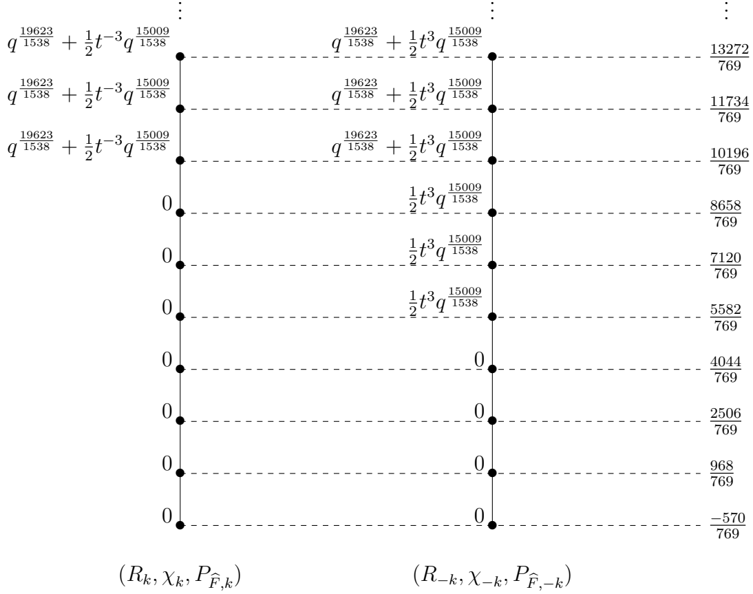
FIGURE 8. Note, d(-Y(\Gamma), [(-5, 5, 8, 9, 1)]) = d(-Y(\Gamma), [(5, -5, -8, -9, -1)]) = -\frac{570}{769} .
