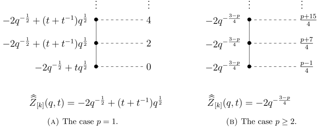
FIGURE 7. The weighted graded root and two-variable series \widehat{\widehat{Z}}_{[k]}(q, t) corresponding to the admissible family \widehat{F} for the one-vertex plumbing \Gamma = \bullet_{-p} with \text{spin}^c structure [-p] . Recall from grading conventions 3.6 that the numbers to the right of the graded root denote the gradings of HF^+(-L(p, 1), [-p]) .
