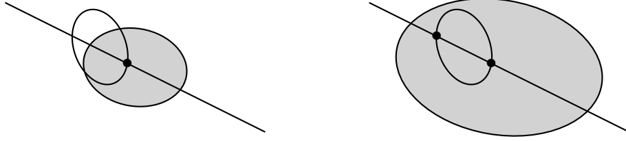
FIGURE 6. A schematic depiction of stabilization. Left: \mathcal{S}_n is represented by the shaded ellipse, \partial\tilde{\mathcal{S}}_i is the unshaded ellipse, and the hyperplane \mathcal{A}_j is the straight line (the actual sets are discrete subsets of the illustration). The intersection \mathcal{S}_n \cap \partial\tilde{\mathcal{S}}_i \cap \mathcal{A}_j is marked by a dot. Right: taking n \gg 0 ensures \partial\tilde{\mathcal{S}}_i \subset \mathcal{S}_n , and the intersection (two dots) is the same for all sufficiently large n .
