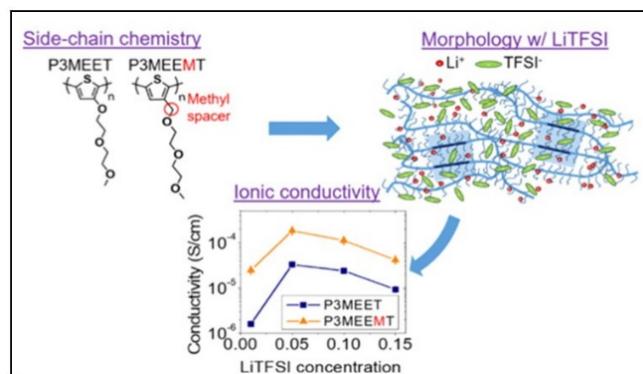
Figure 6. Top-left panel: chemical structures of P3MEET and P3MEEMT . Top-right panel: Schematic representation of LiTFSI distribution within P3MEET/P3MEEMT semicrystalline structure at high concentration of LiTFSI. Bottom panel: P3MEET and P3MEEMT ionic conductivity at 90 °C. Reproduced with permission from American Chemical Society. 81
