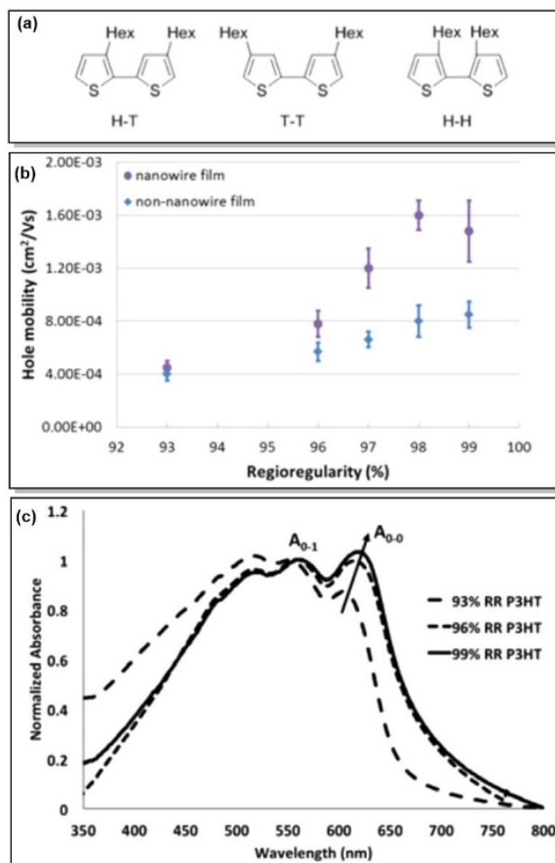
Figure 2. (a) Possible coupling products of P3HT (H-T: head-to-tail, T-T: tail-to-tail, H-H: head-to-head). (b) Correlation between RR and hole mobility for P3HT nanowire and non-nanowire films. (c) UV-Vis absorption spectra for P3HT with various RR%. Reproduced with permission from American Chemical Society. 67
