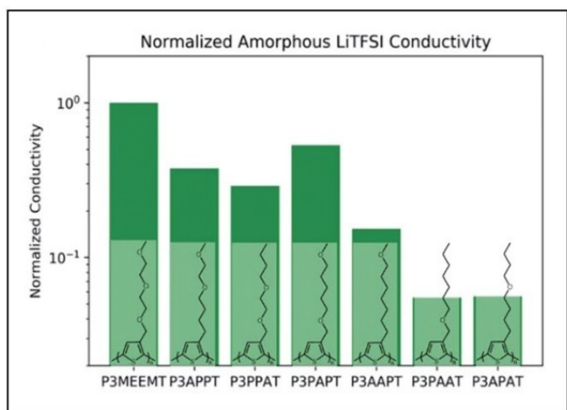
Figure 7. Chemical structures of P3MEEMT , P3APPT , P3PPAT , P3PAPT , P3AAPT , and P3APAT along with the calculated ionic conductivity values for amorphous polymer samples, normalized with the respective polymer dissociation energies, and further normalized against the P3MEEMT performance. Reproduced with permission from Royal Society of Chemistry. 82
