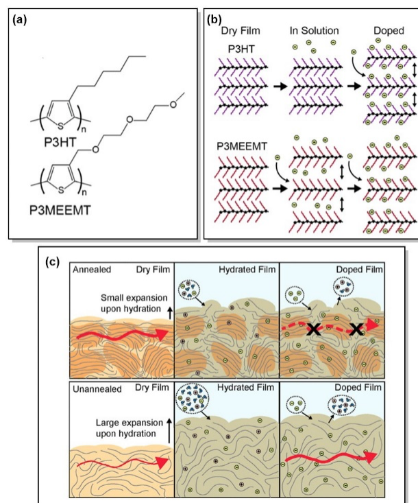
Figure 5. (a) Chemical structures of P3HT and P3MEEMT . (b) Schematic of structural changes in P3HT and P3MEEMT in solution and upon electrochemical doping with P3MEEMT exhibiting a lattice expansion in solution, and the P3HT lattice expanding only upon electrochemical doping (green circles represent anions). (c) Schematic representing charge mobility in annealed and unannealed P3MEEMT (red arrows indicate charge carrier migration through the film). In the dry state, the annealed film is more crystalline and has higher mobility compared to the unannealed sample. When hydrated, the unannealed film swells more and uptakes more electrolyte solution. Lower mobility in the annealed P3MEEMT is assigned to heterogeneity in film swelling. Reproduced with permission from American Chemical Society. 79
