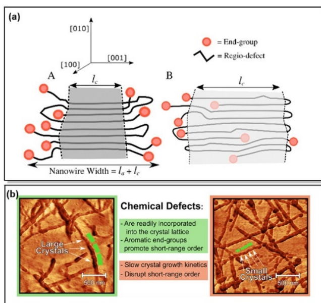
Figure 3. (a) Proposed P3HT nanowire structures with (A) complete or (B) partial defect expulsion, where the darker grey area corresponds to the higher crystallinity region. (b) Young's modulus (AFM scans) of P3HT nanowires with lower (left panel) and higher (right panel) defect concentration. Reproduced with permission from American Chemical Society. 70
