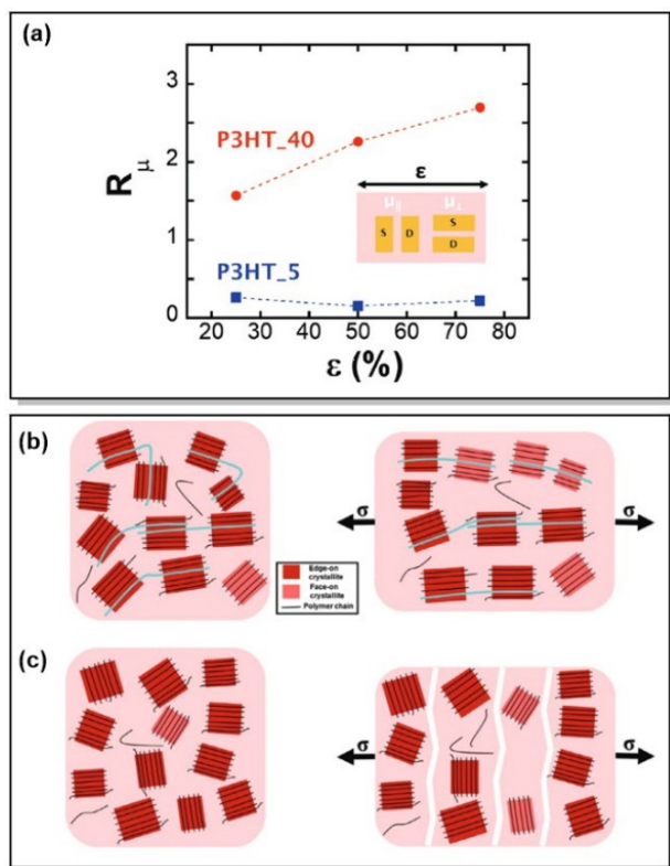
Figure 11. (a) Anisotropy in the field-effect mobility ( R_{\mu} ) of transistors utilizing P3HT_40 and P3HT_5 thin films, as a function of strain. Schemes of unstrained and strained (b) P3HT_40 and (c) P3HT_5 , highlighting the role of tie chains between the crystallites on polymer morphology upon strain. Reproduced with permission from Wiley. 91
