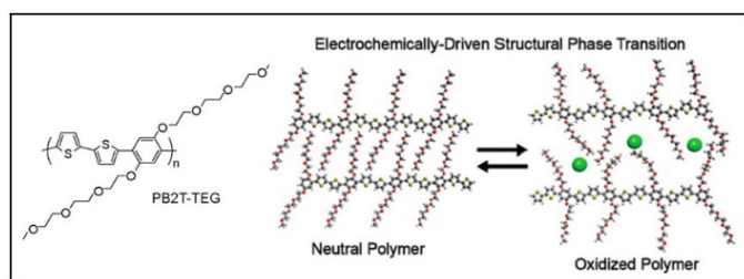
Figure 8. Chemical structure of PB2T-TEG along with the uncovered unzipping/zipping mechanism for ion insertion. Reproduced with permission from American Chemical Society. 83
