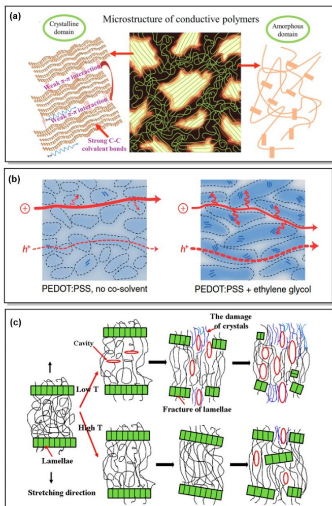
Figure 1. (a) Microstructural features in CPs. Reproduced with permission from Wiley. 25 (b) Morphological changes along with associated hole and ion transport in PEDOT:PSS (Scheme 1). The arrows correspond to the intracrystalline hole transport. Reproduced with permission from Springer Nature. 26 (c) Strain-induced microstructural changes in a semicrystalline polymer. Reproduced with permission from Elsevier. 27
