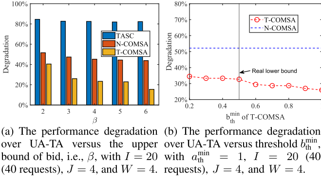
Fig. 8. The performance degradation over UA-TA under different bid distributions and bid threshold b_{th}^{\min} .
