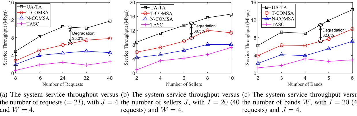
Fig. 7. The system service throughput under different schemes with varied network factors.
