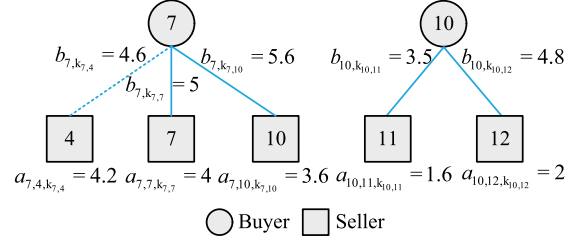
Fig. 4. An example of Subroutine2. The solid lines represent the winning pairs, and the dot line represents the losing pair.
