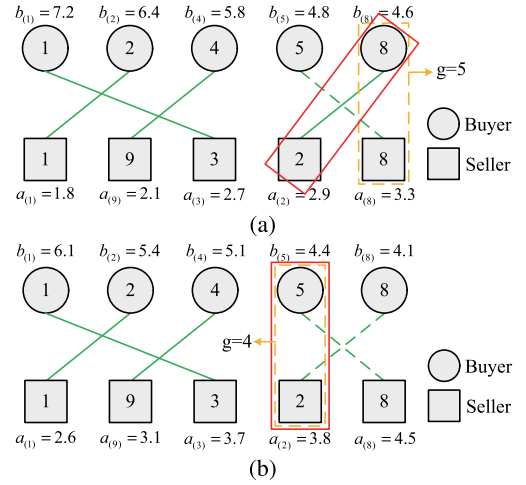
Fig. 5. Two examples of Subroutine3. In each subfigure, the dash rectangle marks the pair (i_g, j_g) with the maximum g that b_{(i_g)} \geq a_{(j_g)} , the solid rectangle marks the boundary (\hat{x}, \hat{y}) , the solid lines denote the winning pairs, and the dash lines denote the losing pairs.
