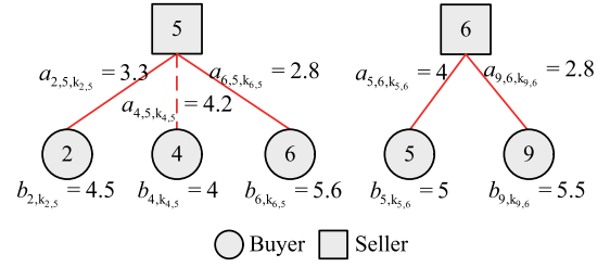
Fig. 3. An example of Subroutine1. The solid lines represent the winning pairs, and the dash line represents the losing pair.
