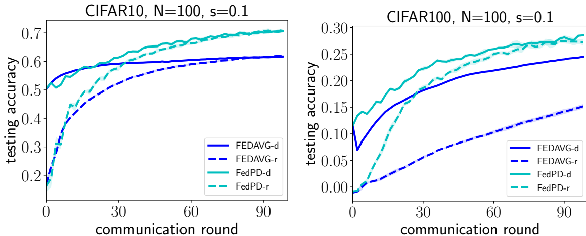
Figure 1: Performance of baseline methods when initialized with a single FFGB-DISTILL step (" \langle \text{alg} \rangle -d") and randomly initialized (" \langle \text{alg} \rangle -r"). Here FEDPD is a synonym for FEDDYN as these two methods are proved to be equivalent.
