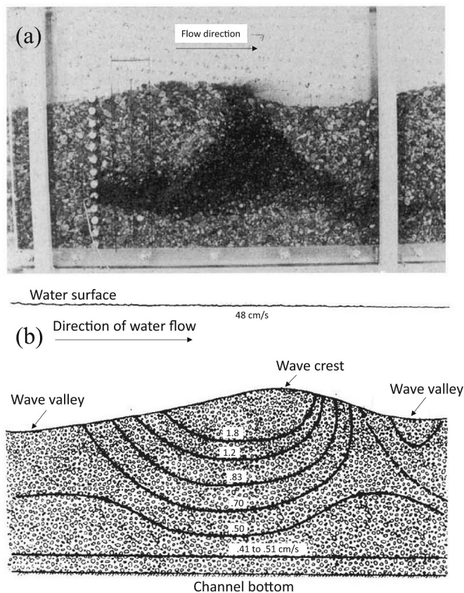
Fig. 6. (a) Typical tracer experiments of currents over a bedform showing flushing of the tracer out of the subsurface and discharge of the dye on the leeward side of the bedform. (b) Composite fluid dynamic diagram showing flow streamlines, zones of surface water inflow and groundwater discharge, and the magnitude of porewater velocities. Scale marker = 6 cm. Taken from Thibodeaux and Boyle (1987).
