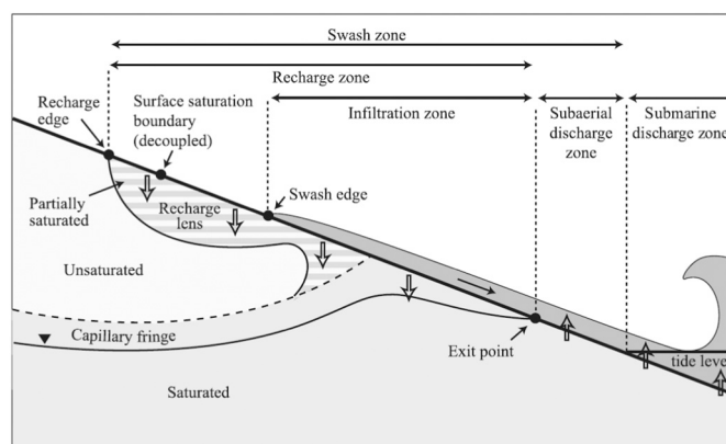
Fig. 3. Schematic of surface water and groundwater levels in the swash zone. The locations of the infiltration, recharge, and discharge zones move across the beachface with tide. Adapted from Heiss et al. (2015).
