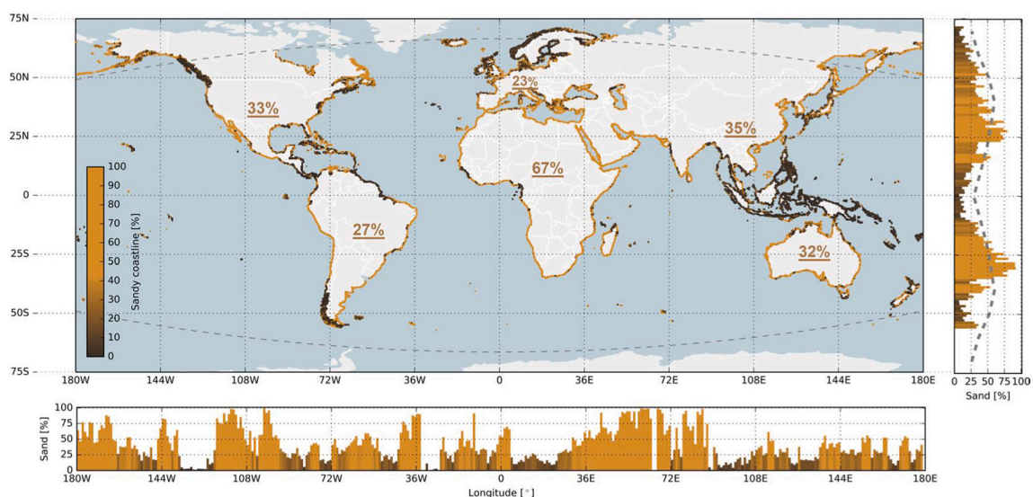
Fig. 1. Global distribution of sandy shorelines; the color contour along the world's shoreline represents the local percentage of sandy shorelines (orange is sand, dark brown is non-sand). The subplot to the right presents the relative occurrence of sandy shorelines per degree latitude, where the dashed line shows the latitudinal distribution of sandy shorelines reported by Hayes and Leatherman (1979). The lower subplot presents the relative occurrence of sandy shorelines per degree longitude. The curved, dashed grey lines in the main plot represent the boundaries of the ice-free shorelines considered in the analysis. The underlined percentages indicate the percent of sandy shorelines for each continent. Reproduced from Luijendijk et al. (2018).
