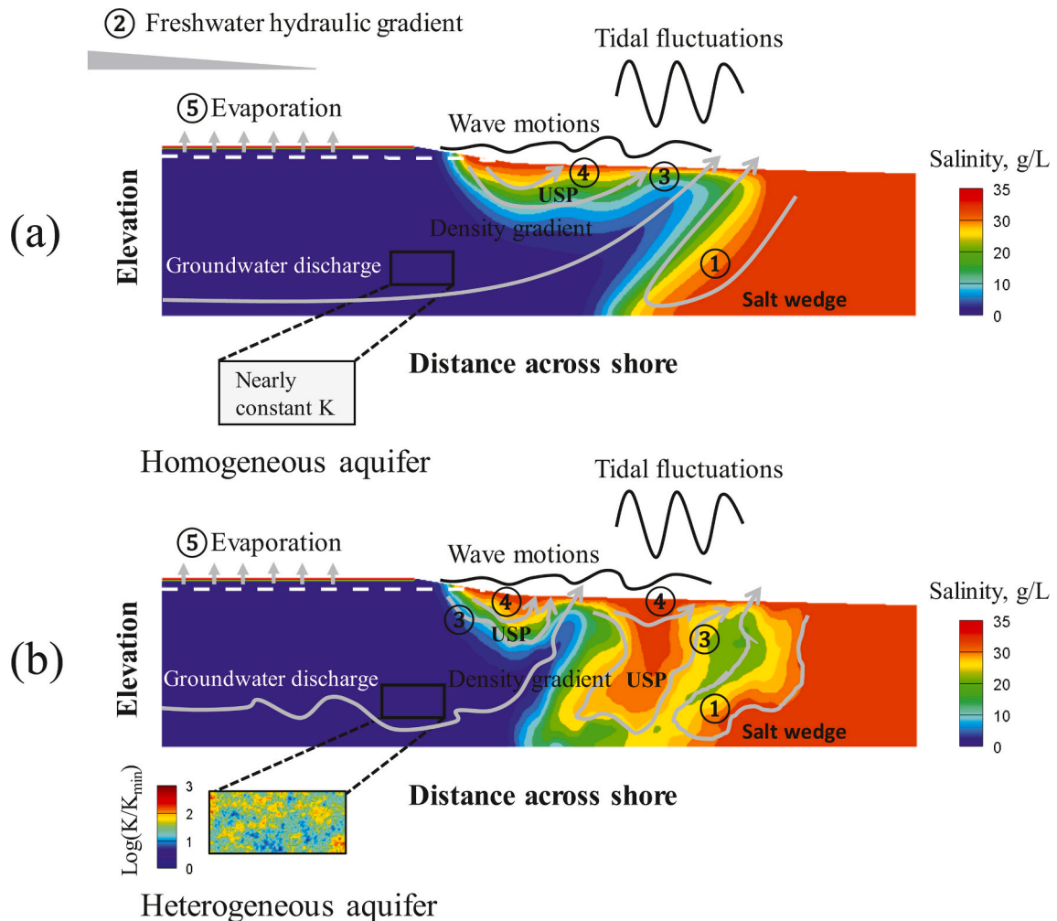
Fig. 2. Schematics of groundwater flow and salt transport processes in (a) homogeneous and (b) heterogeneous coastal aquifers. Process (1) denotes groundwater circulation due to density gradients formed along the dispersed interfaces between fresh water and saltwater. Process (2) denotes inland freshwater hydraulic gradient, driving terrestrial groundwater discharge seaward. Processes (3) and (4) denote groundwater flow driven by tides and waves, respectively. Process (5) represents upward pore-water flow driven by evaporation. The effects of heterogeneity on creating complex flow patterns and salt fingers is illustrated in panel b.
