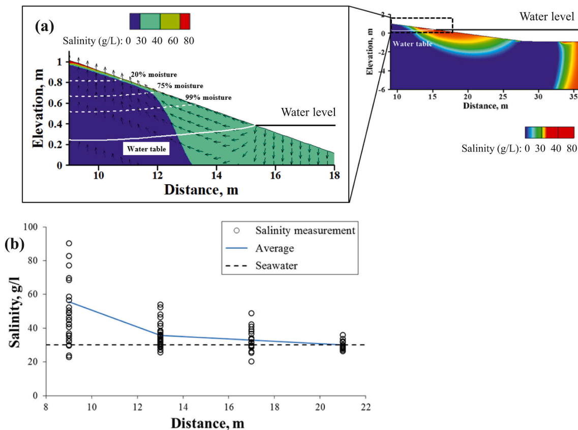
Fig. 4. (a) Simulated salinity contour. White dashed lines denote moisture content (percentage by volume) and the white solid line denotes the groundwater table. The velocity vectors indicate only the pore-water velocity direction, but not its magnitude. Also, note that due to the exaggeration of the vertical scale, the velocity vectors do not appear perpendicular to the beach surface (as the beach slope was visually increased). Extremely high pore-water salinity was measured near the upper intertidal zone in the top 5 cm; in contrast, pore water salinity at other depths and/or locations was almost the same as seawater. The simulated salinities indicate that a high saline layer formed along the beach surface due to evaporation. (b) Observed salinity profile in the top 5 cm layer of the beach sampled ~every 2 h over complete tidal cycles for 7 discontinuous days over summer period. Two values 160 g/l and 220 g/l are not reported in the fig. for visual clarity, but were considered when calculating the average value. Adapted from Geng et al. (2016a).
