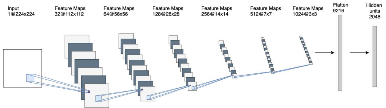
FIGURE 5. Encoder structure of the CNN autoencoder for cropped face image, each convolution layer with 3 \times 3 convolutional kernel.
