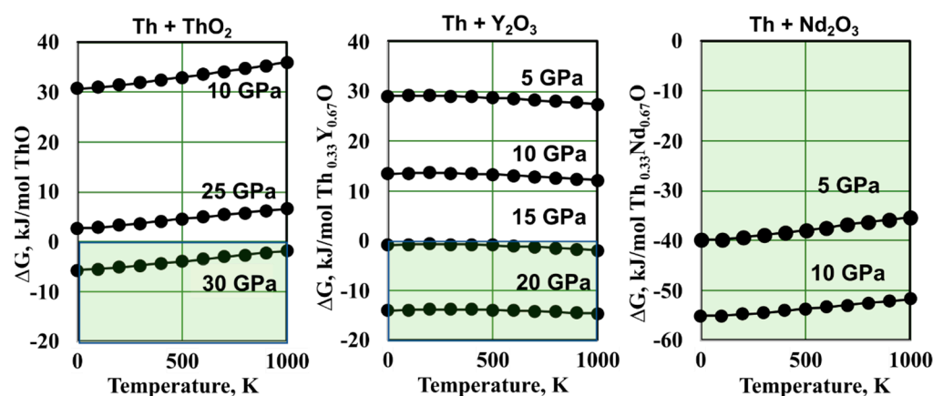
Figure 5. New computational results: free energy for reactions of ThO and (Th,RE)O formation from Th metal, ThO 2 , Y 2 O 3 , and Nd 2 O 3 . The fields of thermodynamic stability of the rocksalt solid solutions are marked in green.
