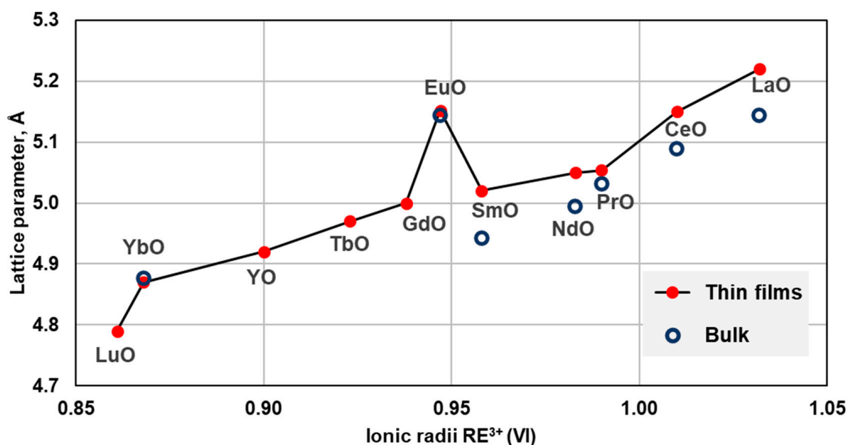
Figure 4. Cell parameters of rocksalt-type REO from high-pressure synthesis and thin films. The symbol sizes exceed reported uncertainties. Reported cell parameter for HoO film ( a = 5.04 Å) is not included in the plot as a possible outlier. The references are listed in Table 2.
