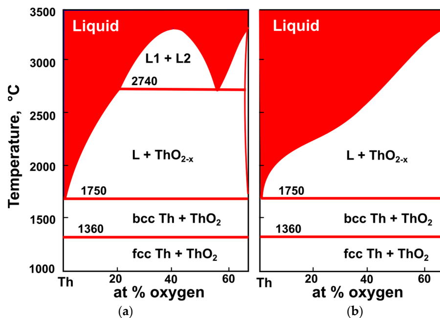
Figure 2. Thermodynamic assessments of Th-O system (a) after McMurray et al. [55]; (b) after Bergeron et al. [56].
