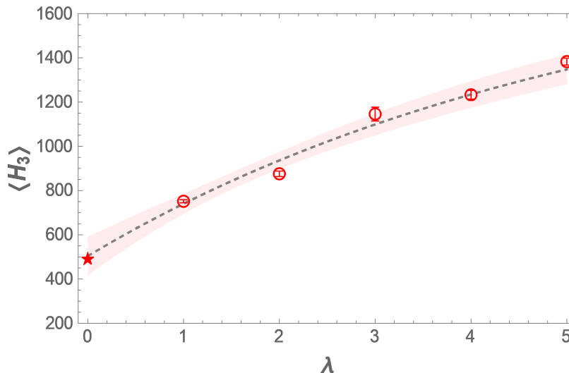
FIG. 4: Expectation value (in MeV) of H_3 , obtained by combining the plots in Fig. 3 with 2\sigma prediction bands. Actual values have 95% chance of lying within bands. Noiseless quantum simulation result is indicated by the star symbol for comparison.
