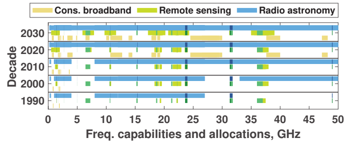
Fig. 1: Spectrum capabilities and allocated bands across three stakeholders: remote sensing, consumer broadband (including mobile cellular and LEO satellite) and radio astronomy.
