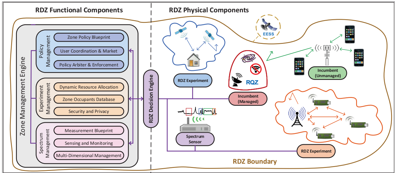
Fig. 4: Overview of a Radio Dynamic Zone illustrating the key functional components in charge of managing the zone, active experimentation within the zone, potential incorporation of Radio Quiet Zones, and protection of incumbents and experimenters.
