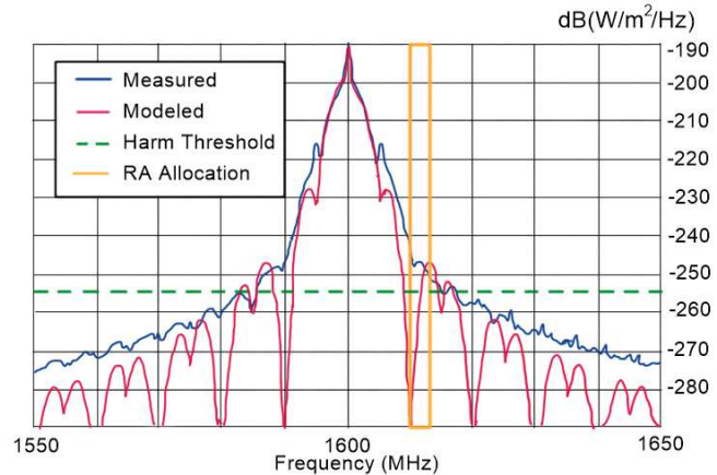
Fig. 3: Modeled and measured spectrum of GLONASS transmissions showing its unintended impact on radio astronomy.
