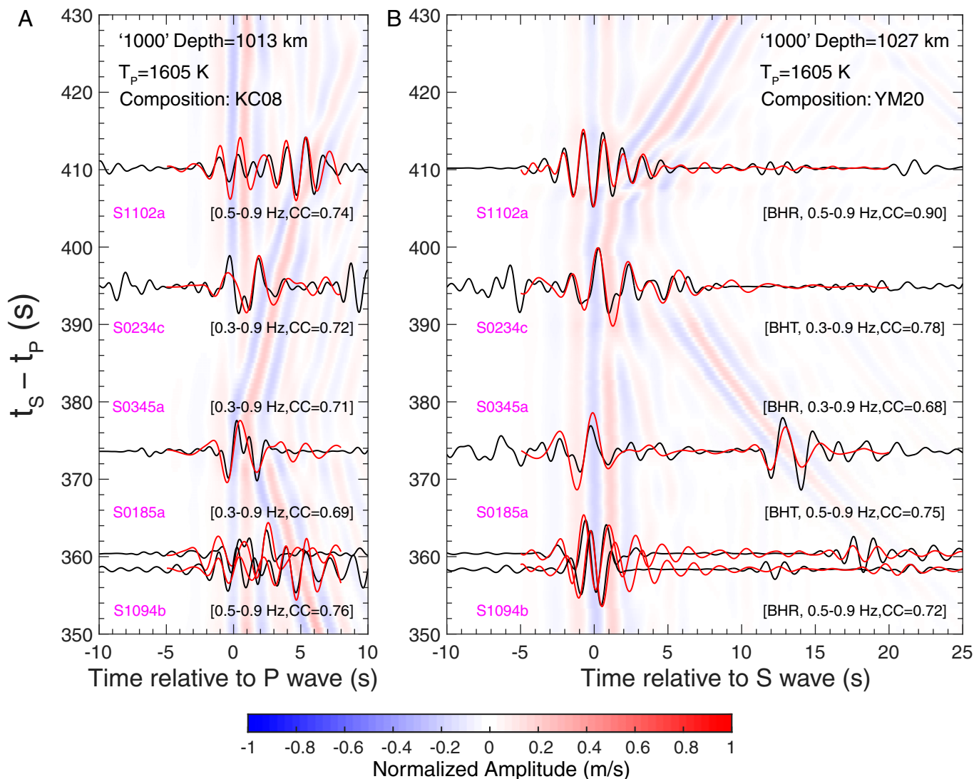
Fig. 2. InSight seismic observations of P and S triplications and synthetic waveform fits. Polarization filtered (A) P waveforms on the vertical component (BHZ) and (B) S waveforms on the transverse (BHT) or radial (BHR) components are shown in black curves. We selected either the BHT or BHR component based upon the SNR of the S waves. The bandpass filters for each waveform are listed to the right. Red curves denote the synthetic waveforms from the best-fitting models, with the CCs listed to the right. The parameters of the best-fitting models are shown on the top, and KC08 (46) and YM20 (20) represent the assumed composition models. Background colors denote the amplitudes of P-wave synthetics on the BHZ component and S-wave synthetics on the BHT component, assuming a 30-km source depth. We only consider the fits between data and synthetics in specific time windows (–5 to 8 s for P waves and –5 to 20 s for S waves) to avoid contamination from other seismic phases and noise. Note that the time windows for the S waves in S0185a and S1094b events are extended to account for possible later arrivals of triplications.
