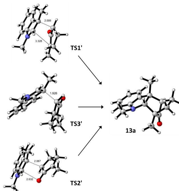
Figure 2. DFT located transition structures (TS') leading to formation of the minor isomer 13a . Relative free energies are shown in Figure 3.
