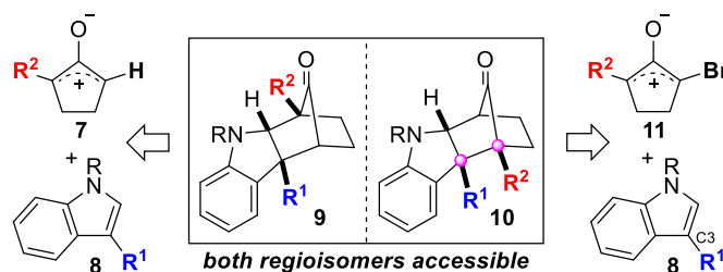
Scheme 1. A) Standard regioselectivity for annulation reactions of oxyallyl cations. B) Regiodivergent synthesis of stereodefined, vicinal, quaternary centers by (3+2) annulation reactions of oxyallyl cations.
