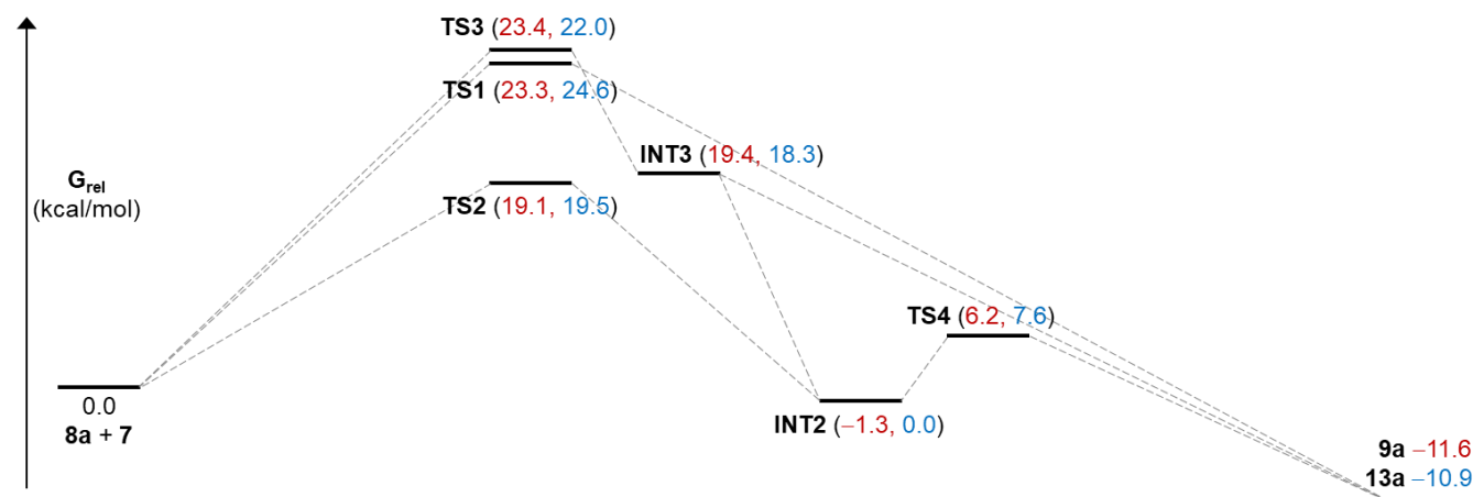
Figure 3. Relative free energies (DFT/B3LYP-D3/def2-tzvp/TFE) for species illustrated in Figures 1 and 3. Numbers in red are for the major stereoisomer 9a and in blue for minor regioisomer 13a .
