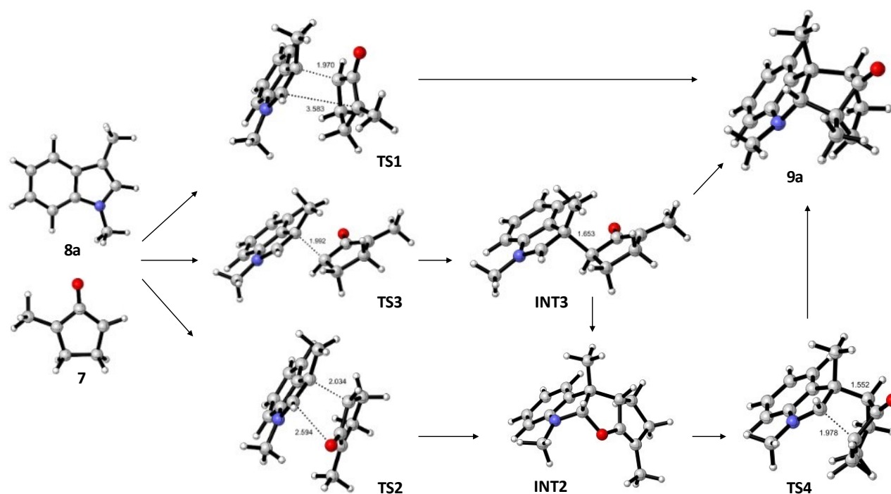
Figure 1. DFT located transition structures (TS) and intermediates (INT) leading to formation of the major isomer 9a . Relative free energies are shown in Figure 3.
