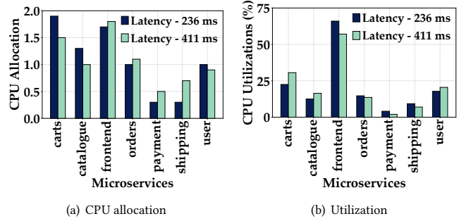
Figure 6: (a) Total CPU allocation of 7.5 distributed among different microservices of SockShop. (b) CPU utilization.
