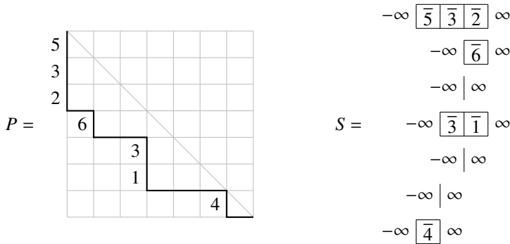
Figure 6. Example of the bijection P = P_T \leftrightarrow T \leftrightarrow S = T^R \circ \sigma in Proposition 6.1.1, with m = 1 , p = 1 - \epsilon , \sigma = w_0 . Letters in S are ordered \bar{1} > \bar{2} > \dots . We see \text{dinv}_1(P) = h_{w_0}(S) = 6 .
