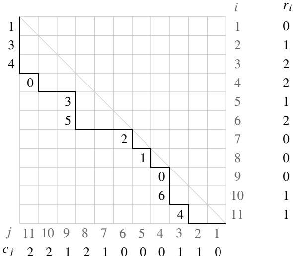
Figure 1. A path \lambda and partial labelling P \in \mathbf{L}_{11,2}(\lambda) , with \text{area}(\lambda) = 10 , \text{dinv}(P) = 15 , x^{\text{wt}_+(P)} = x_1^2 x_2 x_3 x_4^2 x_5 x_6 and x^{\text{wt}(P)} = x_0^2 x_1^2 x_2 x_3^2 x_4^2 x_5 x_6 .
