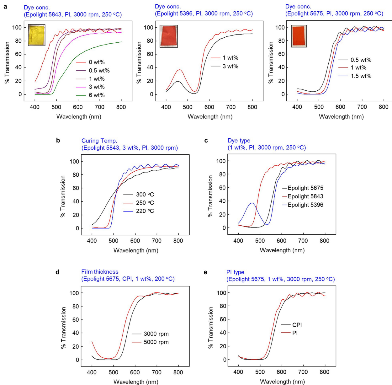
Extended Data Fig. 5 | Optimization of optical transmission characteristics of absorber interlayers. a-e , Optical transmission spectra obtained from absorber layers with varying concentrations of dyes dissolved in the PI precursor (a), film curing temperatures (b), types of dye product (c), film
