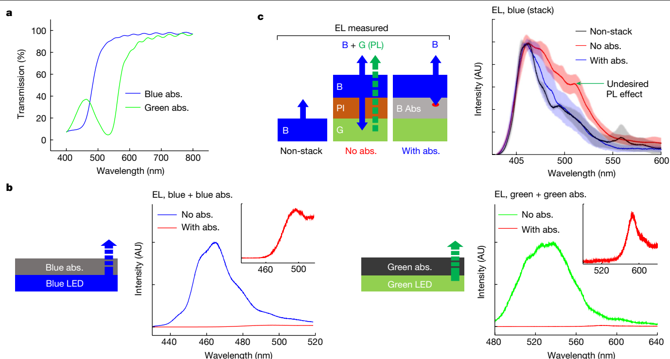
Fig. 3 | Prevention of PL via wavelength-specific, PI-based absorbers.
