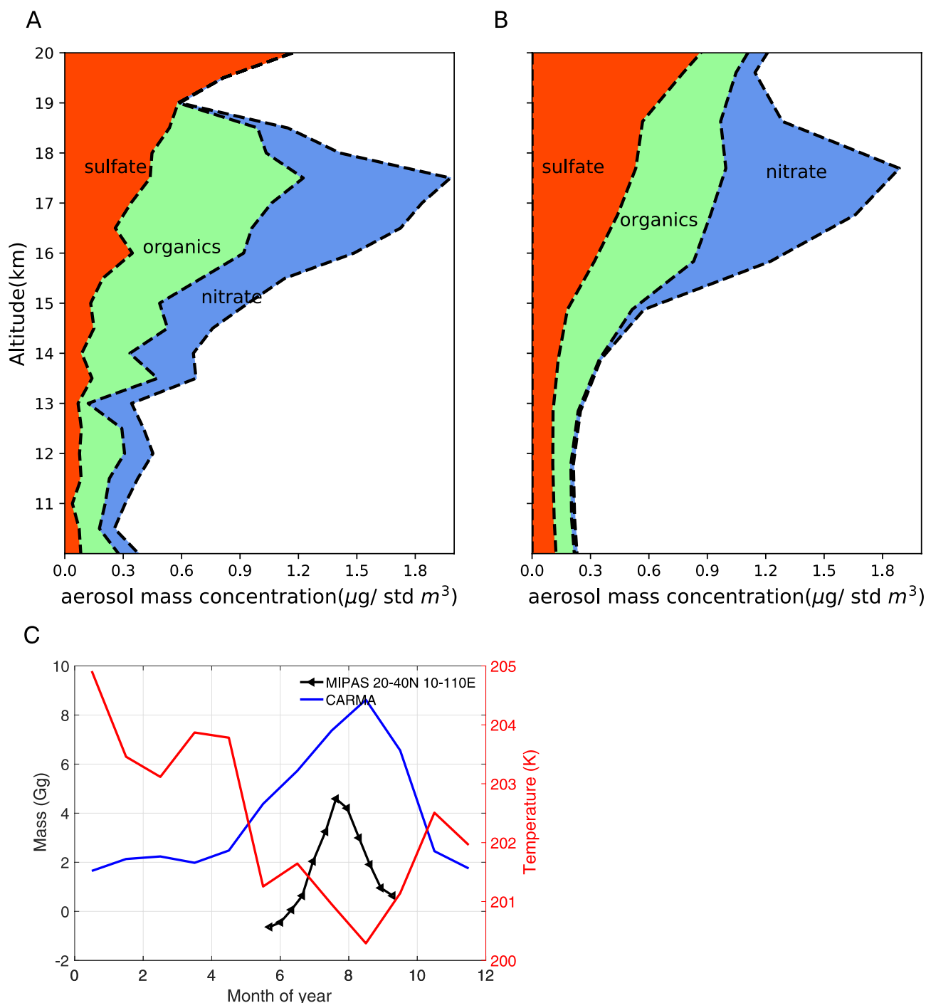
Figure 1. (a) Vertical distribution of the aerosol compositions measured by the Europe Research Council Instrument for the Chemical Composition of Aerosols (ERICA) instrument during the StratoClim field campaign in August of 2017 (Appel et al., 2022; Höpfner et al., 2019). Nitrate, organics and sulfate are denoted by the color-coded stacked regions. Observations are averages of all eight flights in StratoClim field campaign; (b) same as A but for the simulated aerosol composition by Community Earth System Model-CARMA in August of 2017; (c) Simulated monthly mean total nitrate and nitric acid aerosol mass in the upper troposphere and lower stratosphere of Asian monsoon region (20–40°N, 10–110°E, 13–17 km) is shown in the blue line; observations of nitrate in the form of solid ammonium nitrate by the Michelson Interferometer for Passive Atmospheric Sounding (MIPAS) satellite is shown in black line with triangles (Höpfner et al., 2019); simulated temperature vertical distribution is shown by the red line (right axis). Aerosol mass concentrations are in unit of microgram per unit cubic meters in the standard air (std) for all panels.
