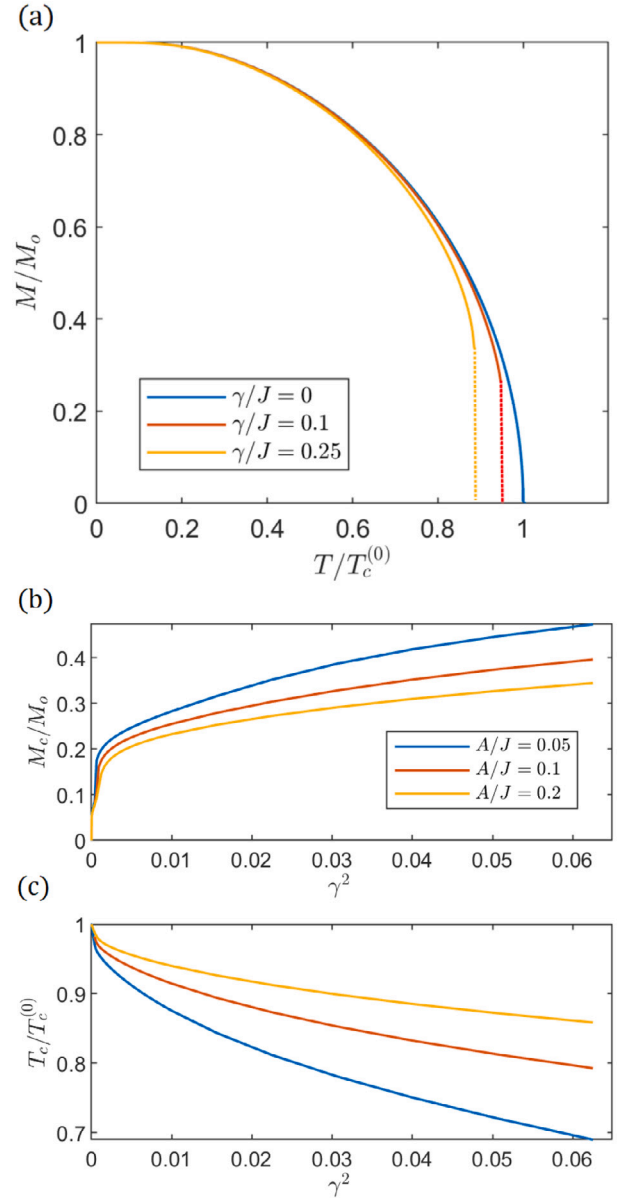
Fig. 2. (a) Magnetization as a function of temperature for several different values of the random fields without an external magnetic field. The dotted lines mark the critical points where the solutions end and the first-order phase transition occurs. We have used J = 1 and A = 0.3 , z = 4 . (b) and (c) The critical magnetization and the critical temperature as functions of the strength of the random field for several systems with different anisotropy constants.
