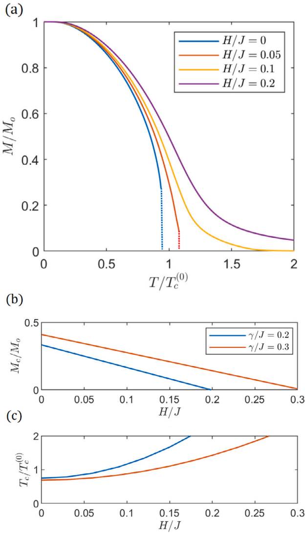
Fig. 3. (a) Magnetization as a function of temperature for several different external magnetic fields. The dotted lines mark the critical points where the solutions end and the first-order phase transition occurs. A = 0.2 , z = 4 , and \gamma = 0.1 . (b) and (c) The critical magnetization and the critical temperature as functions of the external magnetic field for several different random fields. A = 0.2 , z = 4 .
