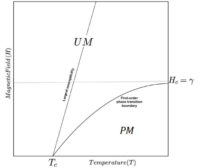
Fig. 4. The phase diagram of a two-dimensional magnetic system with a random field (based on the data presented in Fig. 3c). The solid black line represents the first-order phase transition from the uniform magnetization phase (UM) to a paramagnetic state (PM). The dotted line represents the maximum susceptibility for the uniform magnetization. The critical magnetic field scales with H_c = \gamma .
