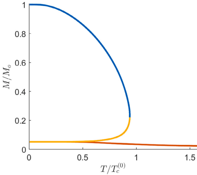
Fig. 1. The complete solutions of M as a function of temperature are calculated from Eqs. (13) and (14). The section with the blue line is the equilibrium ferromagnetic state while the other two sections are not stable states. The section with the yellow color has higher free energy compared to the blue line and the section with the orange color has a negative effective energy gap. We have used J = 1 , z = 4 , A = 0.2 , H = 0 and \gamma = 0.1 .
