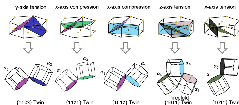
Figure 14. Schematics of the formation process of seven hcp ( \alpha )-variants and the corresponding twins as a result of the \omega \rightarrow hcp martensitic phase transformation in MD simulations by Zahiri et al. [55]. The two \{11\bar{2}0\}_{\omega} planes are highlighted in light blue and black in the \omega unit cells and five different \{01\bar{1}1\}_{\omega} planes are highlighted in purple, blue, green, pink, and dark green in the \omega unit cells, which directly transform into basal planes of \alpha_1 \sim \alpha_7 variants. Reprinted with permission from Ref. [55]. 2021, the American Institute of Physics.
