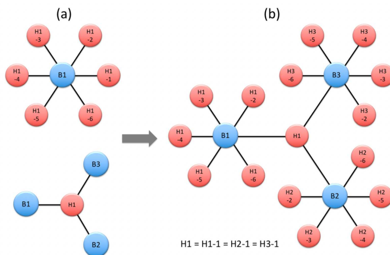
Figure 5. The phase transition graph approach used by Gao et al. [48] for bcc–hcp transformation. (a) Local structures. (b) The global structures generated by combining multiple local structures. Reprinted with permission from Ref. [48]. 2020, the American Physical Society.
