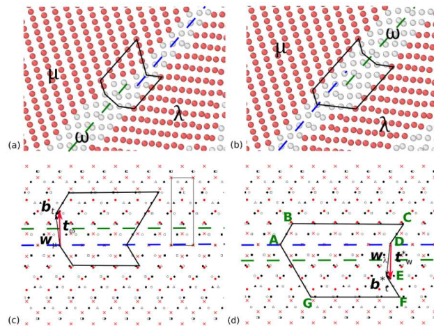
Figure 11. (a,b) Dissociated segments of \{11\bar{2}2\} boundary and Burgers circuits around a pair of steps in MD simulation by Ostapovets et al. [102]. (c,d) Burgers circuits from (a) and (b), reproduced in trichromatic complexes. The twin crystal ( \mu ), matrix crystal ( \lambda ) and omega-phase crystal ( \omega ) are marked by black, white and red symbols, respectively. The net Burgers vector of the pair of steps equals to that of the b_{3/3} disconnections. Reproduce from ref. [102] with permission from Elsevier.
