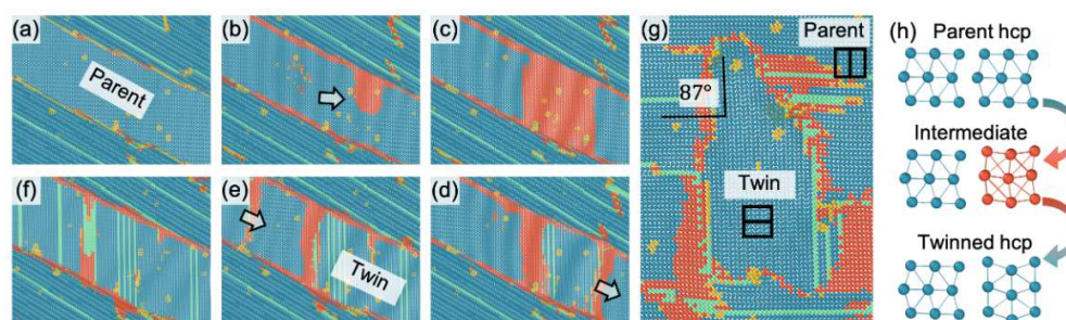
Figure 6. The MD simulation by Ombogo et al. [50] showing the \{10\bar{1}2\} extension twin formation through (a,b) hcp-to-tetragonal and (c,d) tetragonal-to-hcp martensitic phase transformations in Mg. The two formed \{10\bar{1}2\} twin boundaries (e) migrate quickly and (f) react with each other and result in a few layers of fcc phase. (g) A close-up view shows the \{10\bar{1}2\} twin orientation of the newly formed hcp phase with the parent hcp phase: 87° misorientation across a common \langle a \rangle -axis. (h) Schematic illustration of the twin formation process. Hcp, bcc-like (tetragonal), fcc, and amorphous structured atoms are shown by cyan, red, green, and yellow colors, respectively. The long lines of green atoms are partial stacking faults.
