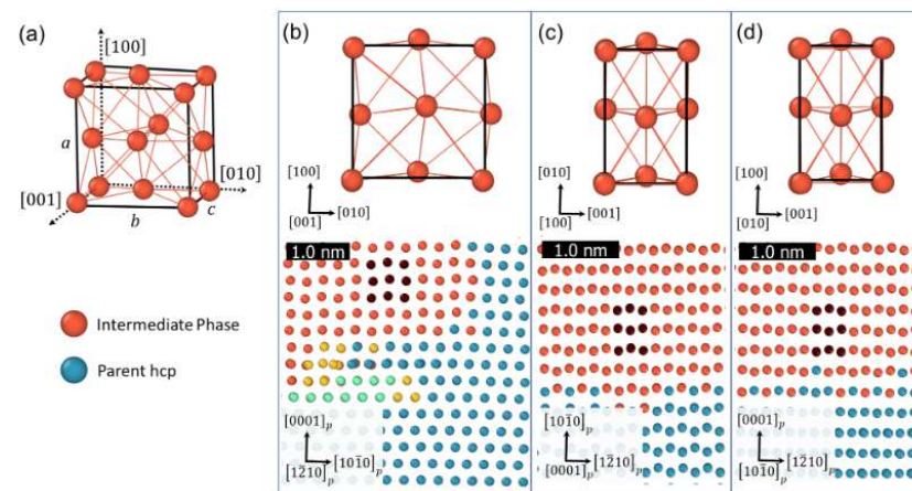
Figure 7. (a) A unit cell of the metastable tetragonal phase extracted from the MD simulation by Ombogo et al. [50]. Its different projections along (b) [001] , (c) [100] , and (d) [010] directions. Below each projection of the unit cell are thin slices of the MD simulation (b) viewed along the common \langle a \rangle -axis of the \{10\bar{1}2\} extension twin, (c) projected onto the parent basal plane, and (d) projected onto the parent prismatic plane, in which atoms in one tetragonal unit cell are highlighted in black [50].
