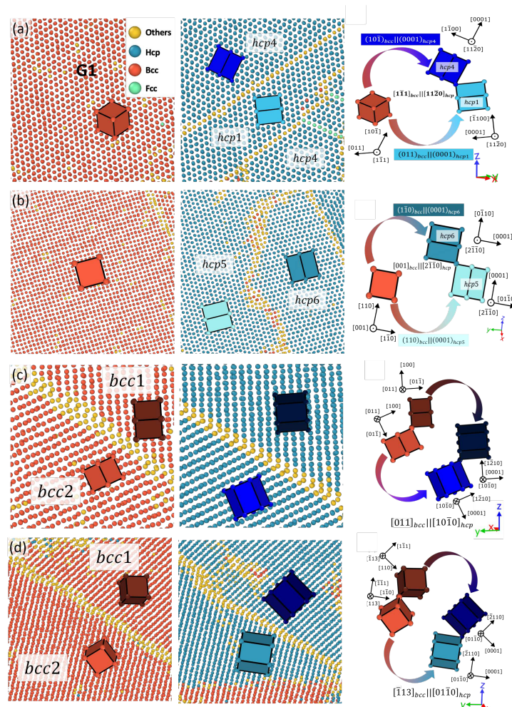
Figure 12. The formation process of four transformation twins in MD simulations of bcc-hcp phase transformation by Zahiri et al. [112]. In the same grain, (a) under x-tension, the phase transition forms a \{10\bar{1}1\}_{hcp} twin; (b) under x-compression, the phase transition forms a \{10\bar{1}2\}_{hcp} twin. In a \{112\}_{bcc} twinned grain, (c) under x-tension, the phase transition forms a \{11\bar{2}2\}_{hcp} twin; and (d) under x-compression, the phase transition forms a \{11\bar{2}1\}_{hcp} twin. Adapted with permission from Ref. [112]. 2022, Elsevier.
