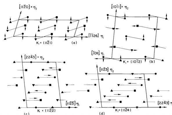
Figure 1. The arrows represent the possible atomic shuffles accompanied lattice shear for (a) \{11\bar{2}1\} , (b) \{10\bar{1}2\} , (c) \{11\bar{2}2\} and (d) \{11\bar{2}4\} twinning modes in hcp Ti. Different symbols represent atoms from different crystallographic planes that are parallel to the plane of the figure. Motif pairs of atoms are linked together and assumed to move together. Reprinted with permission from Ref. [7], 1970, Elsevier.
