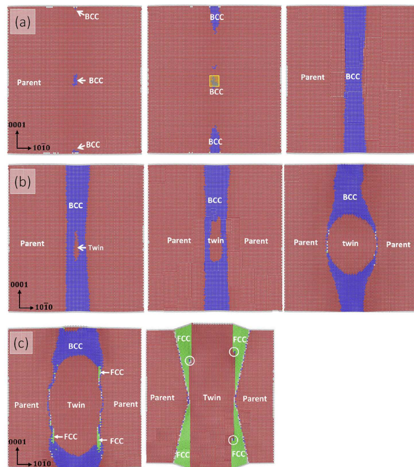
Figure 8. The MD simulation of Ti by Chen et al. [49] revealed the transitory bcc phase during the nucleation of \{10\bar{1}2\} deformation twin. Based on common neighbor analysis, hcp, bcc, and fcc atoms are shown in red, blue, and green, respectively. Reprinted with permission from Ref. [49]. 2019, Elsevier.
