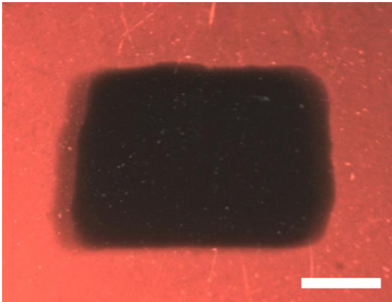
FIGURE 10: A: PROFILOMETRY RESULTS FOR A FILM PRINTED ON KAPTON ON A SILICON WAFER WITH THE FOLLOWING PARAMETERS: PRESSURE – 20 PSI, DEPOSITION HEIGHT – 3MM, STROKE – 55%. RESULTS ARE FROM THE FILM COMPOSED OF 10 SINGLE LAYERS; B: IMAGE OF A FILM COMPOSED OF 8 LINES (PER SINGLE LAYER) AND 5 LAYERS. 60 PSI – 55% STROKE – 1MM DEPOSITION HEIGHT. SCALEBAR = 1MM.
