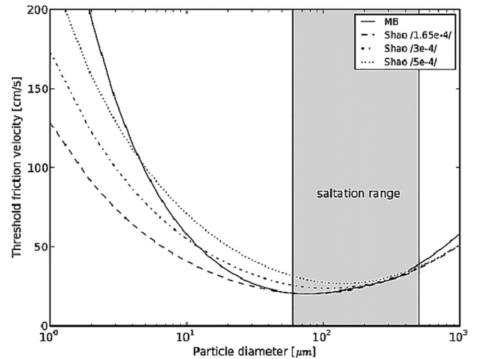
Fig. A1. Threshold friction velocity over a smooth surface calculated with Marticorena and Bergametti (1995; MB) and Shao and Lu (2000) dust emission schemes (taken from Darnenova et al., 2009).
