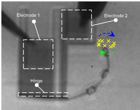
Extended Data Fig. 5 | A microscopic device for measuring the trajectory of one cilium. We at first apply a fixed voltage on the hinge through electrode 1 to make the hinge bend up to about 90°, then apply another oscillating voltage through electrode 2 to actuate the cilium.
