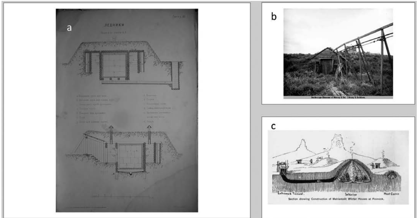
FIG. 4. Historic cellars: a) illustrations including ventilation and wood frame for a Russian lednik (Ледники) design by Zaleskii (1881), b) entrance to natural cold storage plant and pipes from an artificial ice machine at Lomen Elephant Point reindeer processing plant (July 1938. AMRC Ickes Collection: AMRC-b75-175-17, Photographer: Ray B. Dame. Original photograph size: 21.6 cm × 25.4 cm), and c) drawing of a St. Lawrence Island Yupik winter house and cellar (meat cache) in 1874 on Punuk Island by Henry W. Elliott (1886).
