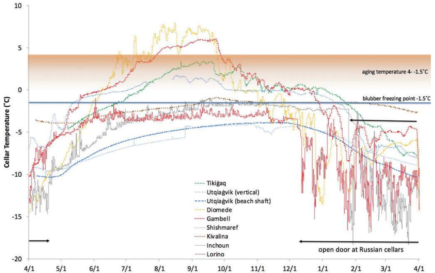
FIG. 9. Annual cellar temperatures as measured in Bering Strait and North Slope communities. Cellar locations indicated in Figure 1.
