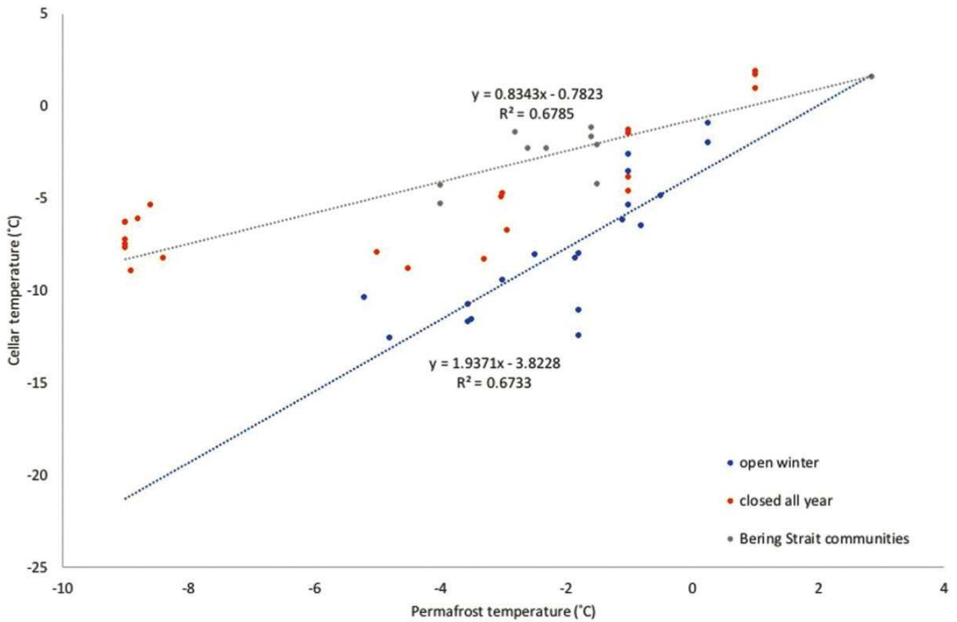
FIG. 11. Mean annual cellar temperature vs. permafrost temperature. Cellars on which the door is left open during the winter are colder than cellars on which doors are kept closed.
