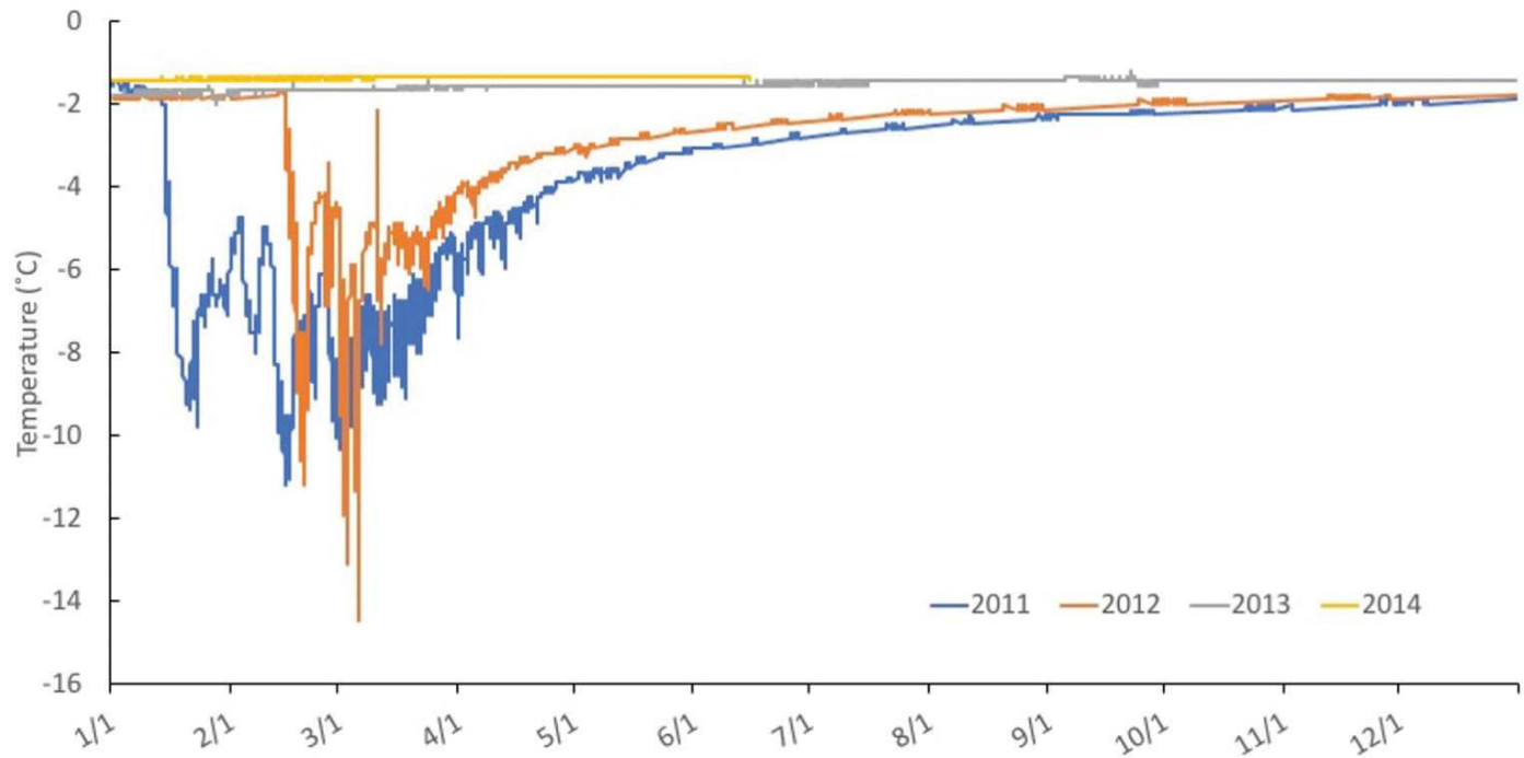
FIG. 12. A four-years door control experiment in an interior Alaska mining tunnel. The tunnel was colder than normal until the end of August when the door was open during winter months of 2011 and 2012 compared to when the door was closed in 2013 and 2014.
