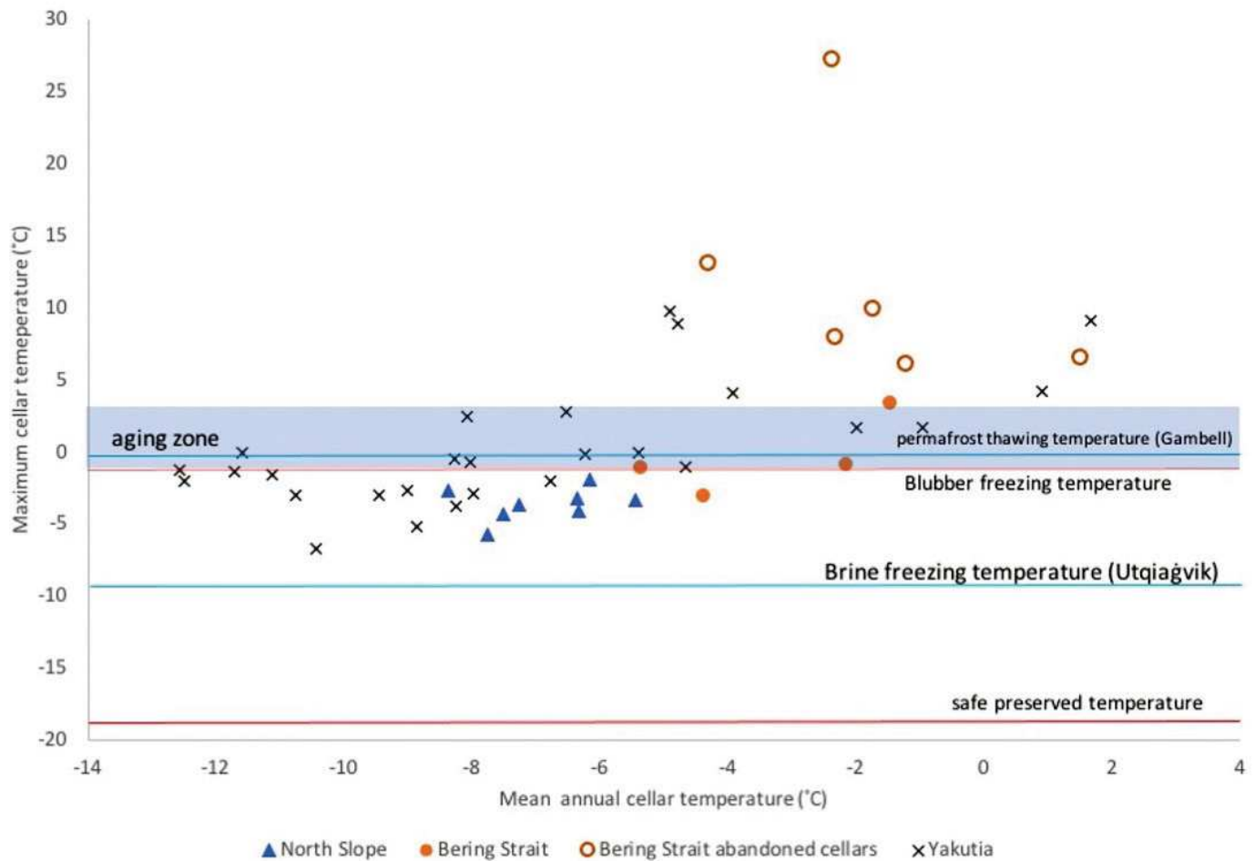
FIG. 13. Maximum vs. mean annual cellar temperature in Bering Strait communities and other areas. Most of the cellars in Bering Strait communities are warmer than the freezing point of whale blubber, however, actively managed cellars may be able to maintain aging temperatures ( -1.5 to +4^{\circ}\text{C} ) during the summer months.
