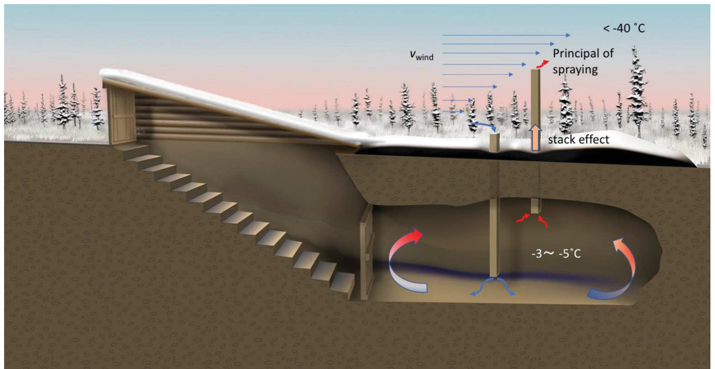
FIG. 7. Natural air circulation within a double ventilation system in Siberian cellars that effectively cools during winter months.
