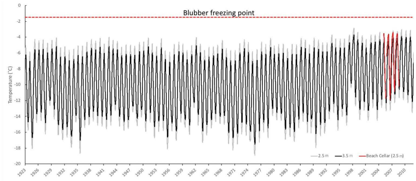
FIG. 10. Reconstructed 88 years of cellar temperatures since 1924 in Utqiagvik (formerly Barrow). Cellar was warming after 1999 event. Red line shows measured cellar temperatures. The dashed red line indicates the freezing point for whale blubber.
