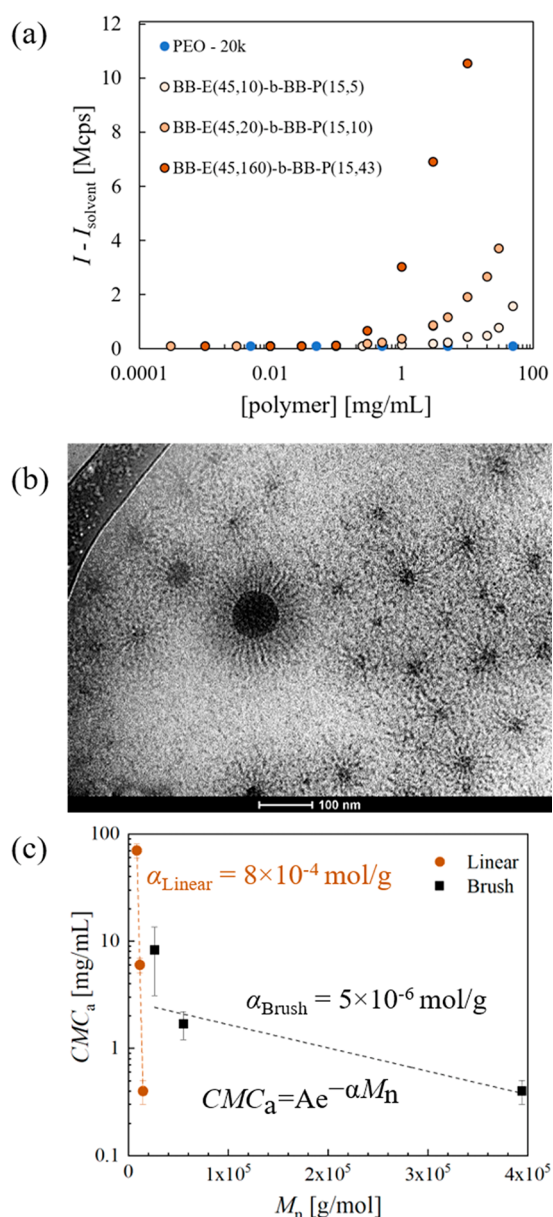
Figure 4. (a) Excess scattering intensity at 37 °C, as a function of polymer concentration. Linear PEO with an M_n = 20 kDa is a negative control for micellization. (b) Cryo-TEM micrograph of BB-E(45,160)-b-BB-P(15,43) at a concentration of 10 mg/mL in aqueous buffer with 40 000 \times magnification. (c) Trend between CMC_a and M_n for linear and bottlebrush poloxamers of similar wt % PEO. Data for linear poloxamers (40 °C) are taken from Alexandridis et al. 59 Data are fit to the exponential function shown on the graph.
