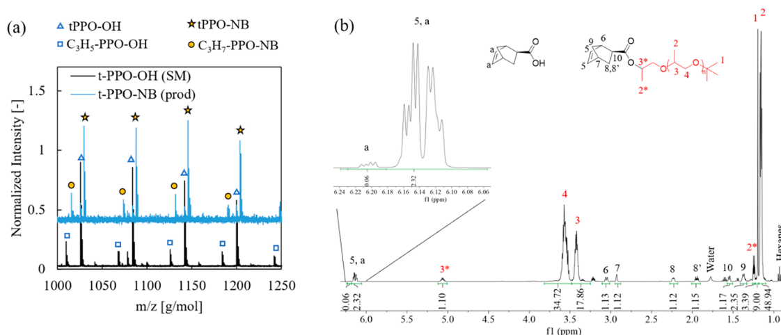
Figure 2. (a) MALDI-ToF spectra of t -PPO-OH and the NB functionalized macromonomer, t -PPO-NB, following the hydrogenation and esterification reactions. M_w = 1210 g/mol and \bar{D} = 1.12 for the SM and M_w = 1330 g/mol and \bar{D} = 1.14 for the product. (b) ^1\text{H} NMR spectrum of the t -PPO-NB macromonomer.
