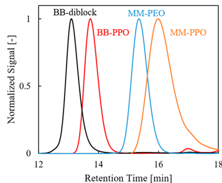
Figure 3. SEC traces with differential refractive index detection of a representative sequential ROMP polymer (BB- E_{45, 20} - b -BB- P_{15, 10} ). The macromonomer traces are included for reference. From the multiangle light scattering detector and a Zimm analysis, the BB-PPO aliquot has a M_w = 11 600 g/mol and \bar{D} = 1.20 and the BB-diblock has a M_w = 55 300 g/mol and \bar{D} = 1.10. Both were within error of the targeted molecular weight. The small peak at ~17 min in the BB-PPO chromatogram is likely a small molecule impurity in the PPO macromonomer, possibly 18-crown-6 ether, that does not impact the subsequent polymerization.
