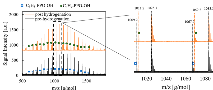
Figure 1. MALDI-ToF spectra of PPO polymer as synthesized via anionic polymerization (black) and post hydrogenation (orange). M_w = 1220 g/mol and \bar{D} = 1.12 for both polymers. The most intense family of peaks in both samples is tert -butyl-PPO-OH ( t -PPO-OH) and is unchanged during hydrogenation. Alkene and alkane \alpha -chain end impurities are labeled accordingly.
