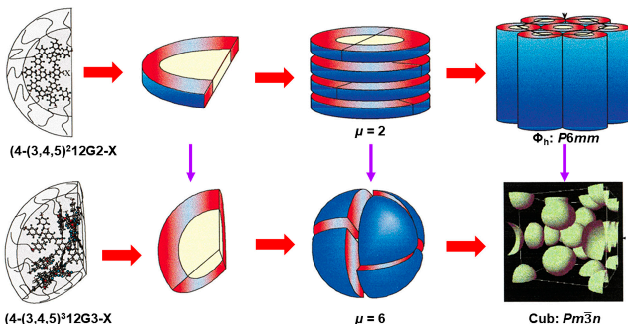
Figure 11. Hierarchical self-organization of the same self-assembling dendron at two different generations. (4-(3,4,5)^2 12G2-X) is second generation (top), and (4-(3,4,5)^3 12G3-X) is third generation (bottom) self-assembling dendron self-assembling columnar and, respectively, spherical assemblies generating columnar hexagonal and cubic Pm\bar{3}n or A15 Frank–Kasper phases [124]. Parts of the Figure were adapted and modified from [124]. Copyright © 1998, American Chemical Society.
