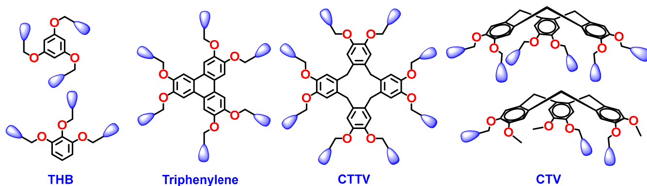
Figure 12. Examples of constitutional isomerism of the focal point. 1,3,5-trihydroxybenzene (THB), triphenylene, cyclotetraveratrylene (CTTV), cyclotriveratrylene (CTV).
