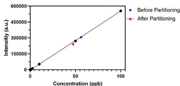
Fig. 2 Calibration curve for the determination of the partition coefficient of \text{HAuCl}_4 using ICP-MS. Gold standards of known concentration were used and diluted by the instrument, with all samples being diluted with 2% \text{HNO}_3 prior to measurement on ICP-MS. The gold standard concentrations were 100, 50, 10, 1, and 0 ppb. Concentrations for standards shown are plotted against raw intensity counts and have arbitrary units (a.u.). All calibration curve measurements were taken at an N = 5 , with measurements for 2.5 mM \text{HAuCl}_4 with 0.1 M \text{LiClO}_4 in water partitioning being taken before and after mixing with 1,2-dichloroethane ( N = 10 ).
