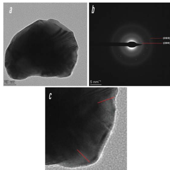
Fig. 4 TEM images of a single gold nanoparticle. (a) Shows a bright field image and (b) shows the selected area diffraction pattern of the gold nanoparticle with their respective miller indices. Additionally, (c) shows the lattice orientation.
