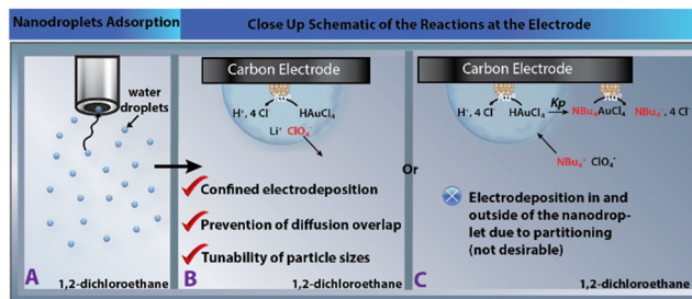
Fig. 1 Schematic representation of the electrodeposition of gold nanoparticles using a quiescent solution. (a) Representation of water nanodroplets suspended in an organic phase where they adsorb into the electrode surface. (b) In the presence of \text{LiClO}_4 , the redox reaction is confined at the water-electrode interface while (c) in the presence of [\text{NBu}_4][\text{ClO}_4] , the reaction happens both inside and outside the water nanodroplet.
