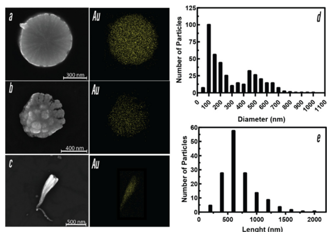
Fig. 3 (a–c) are SEM Images of representative gold nanoparticles (left) electrodeposited using a water-in-oil emulsion. The emulsion was prepared by adding 25 mM \text{HAuCl}_4 and 0.25 M \text{LiClO}_4 to water nanodroplets suspended in 1,2-dichloroethane. EDX mapping was performed showing the presence of gold across each nanoparticle (yellow). (d) The histogram shows a relationship between the number of nanoparticles and size ( N = 402 ) when the nanoparticles look more spherical as presented in a and b. (e) Histogram and SEM images of nanoparticles that are not spherical ( N = 150 ) as presented in c. Nanoparticles were electrodeposited using chronoamperometry. The applied potential was -0.1 V vs. \text{Ag}/\text{AgCl} for 600 seconds. The average droplet radius was 1037 \text{ nm} \pm 238 \text{ nm} ( N = 10 ).
