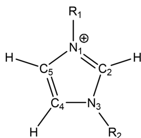
Scheme 1. Numbering system for the imidazolium cation.
