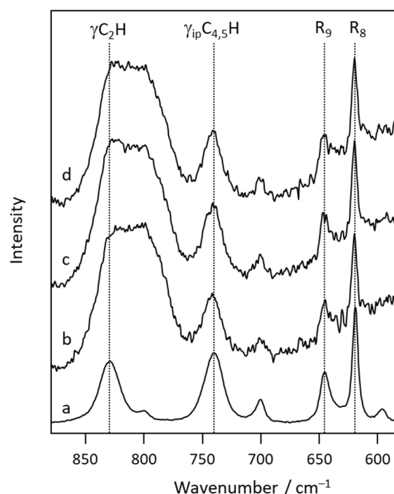
Figure 9. Mid-IR spectra of (a) unconfined [\text{C}_2\text{mim}]\text{FeCl}_4 and [\text{C}_2\text{mim}]\text{FeCl}_4 confined within (b) 8.36, (c) 7.36, and (d) 5.39 nm mesoporous silica.
