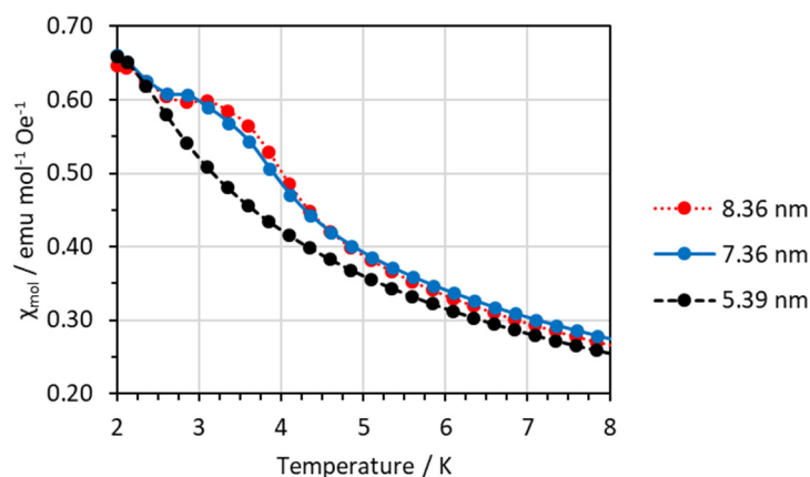
Figure 5. Temperature-dependent, zero-field-cooled molar magnetic susceptibilities for [C_2mim]FeCl_4 confined in silica 1 (red dotted line, 8.36 nm), silica 2 (blue solid line, 7.36 nm), and silica 3 (black dashed line, 5.39 nm).
