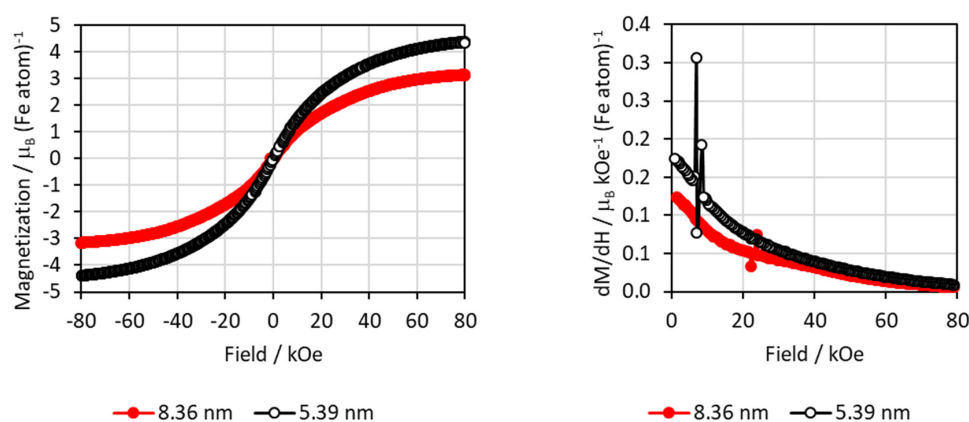
Figure 6. Magnetization (left) and first derivative (right) plots for [C_2mim]FeCl_4 confined within mesoporous SBA-15 silica.
