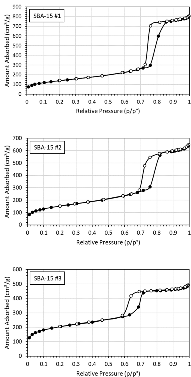
Figure 1. Nitrogen adsorption isotherms for SBA-15 mesoporous silica. Filled and open symbols represent the adsorption and desorption phases of the measurement, respectively.
