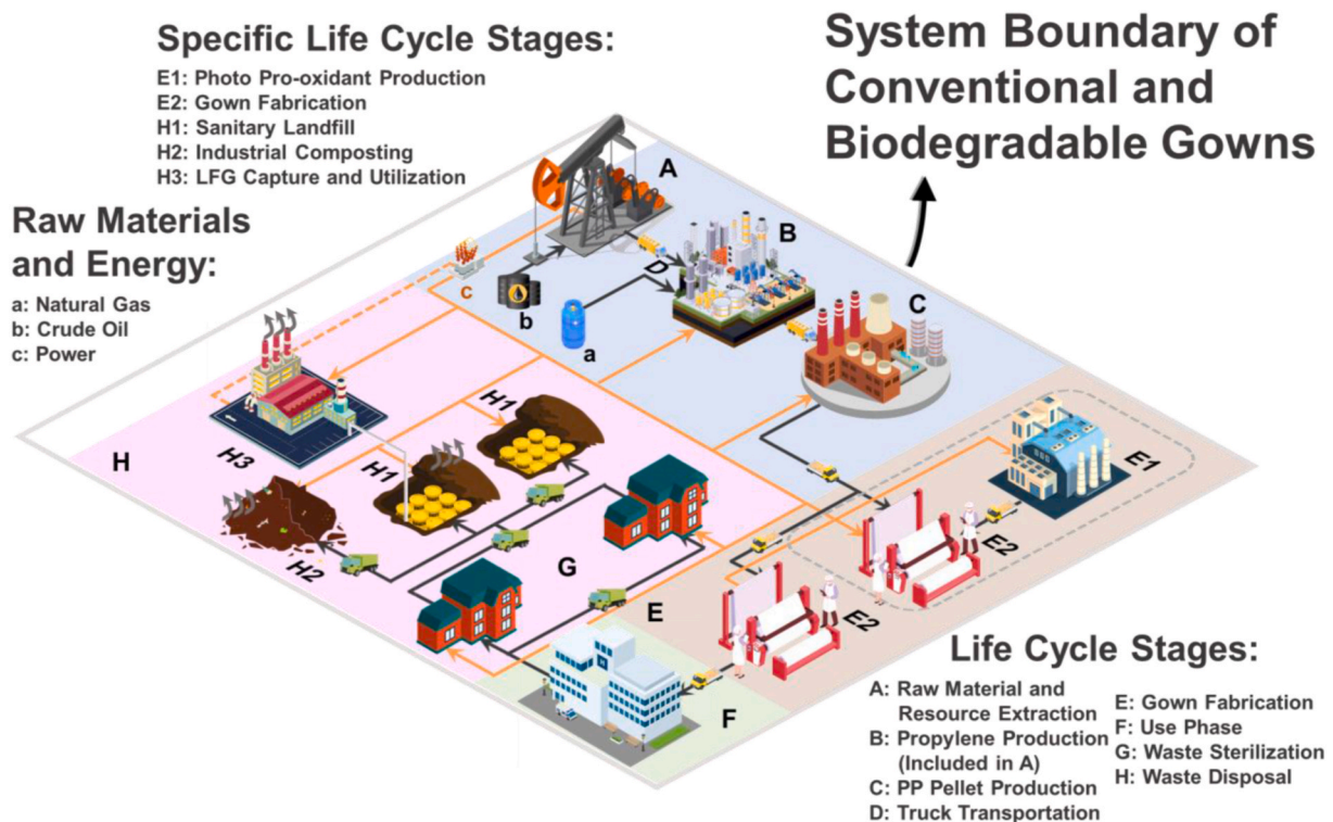
Fig. 1. This comparative LCA study's system boundary corresponds to the conventional and biodegradable gowns. The system boundaries confine the life cycle stages from raw material and resource extraction to EoL disposals, including landfilling for both gowns and biodegradable gown composting. The system boundary of conventional gown waste treated by sanitary landfills covers raw material and resource extraction, propylene production, polypropylene pellet production, truck transportation, gown fabrication, use phase, waste sterilization, and sanitary landfill. Life cycle stages of raw material and resource extraction, propylene production, polypropylene pellet production, truck transportation, photo pro-oxidant production, gown fabrication, use phase, and waste sterilization are all included in the system boundaries of biodegradable gown waste treated by sanitary landfills and industrial composting. These system boundaries also include their specific life cycle stages: LFG capture and utilization for sanitary landfills and industrial composting. The cradle of the conventional and biodegradable gowns are natural gas and crude oil, represented by a and b, respectively, while the c denotes the energy used across the entire gown life cycle.
