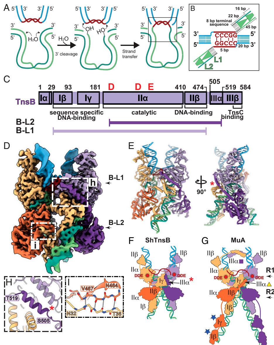
Fig. 1. TnsB STC is a C2-symmetric tetramer with highly intertwined architecture. (A) Schematic of the TnsB transposition mechanism: transposon ends with flanking DNA (green), 5-bp target site (brown), and target DNA (blue). For simplicity, TnsB protomers are not shown. (B) Symmetric strand-transfer DNA substrate is designed to mimic the product of the strand-transfer reaction. The 45-bp part of the transposon left end (LE) includes 1.75 TnsB binding sites (one full binding site, corresponding to 22 bp of L1, and three-fourths of a binding site, corresponding to 16 bp of L2). TnsB binding sites overlap by 1 bp, indicated by green triangles. An 8-bp terminal sequence is colored gray. (C) Domain diagram of TnsB (purple; domain naming conventions follow MuA) and residue positions built for the two different conformations observed: B-L1 and B-L2 (explained further in D). (D) Cryo-EM reconstruction of the TnsB STC. TnsB subunits are referred to according to which TnsB repeat it binds at the transposon end, numbered starting from the target–donor junction. B-L1 is the TnsB monomer that binds the L1 TnsB DNA sequence, and B-L2 binds the L2 site. TnsB monomers are colored shades of purple or orange. B-L1 subunits (light purple and tan) and B-L2 subunits (dark purple and orange) form a C2-symmetric complex. DNA colors are identical with respect to A. (E) Atomic model of the TnsB STC. Two different views are shown; a red asterisk indicates the position of helix III \alpha . (F and G) Architectural schematic of (F) the ShTnsB STC and (G) (PDB ID code 4FCY) the MuA STC from bacteriophage Mu. Helix III \alpha is indicated with a red asterisk, yellow triangle, or purple square. The location of the DDE catalytic triad is indicated with red stars. Blue stars (DNA-binding domains) indicate domains that are present in MuA but not observed in the ShCAST TnsB STC structure. (H and I) Close-up view of intersubunit interactions in the TnsB STC. (H) Domain III \alpha (indicated with a red asterisk) from B-L2 (residues 505 to 519) mediates a three-way interaction in between two B-L1 subunits. (I) B-L1 and B-L2 subunits form stabilizing beta-sheet interactions. Hydrogen bonds are indicated with dashed lines.
