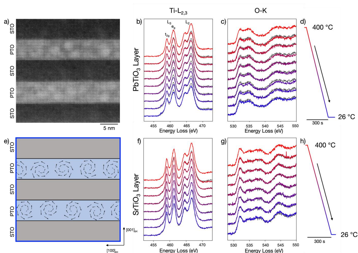
Figure 1. (a) Overview high-angle annular dark-field STEM image of the [010]_{pc} (\text{SrTiO}_3)_{16}(\text{PbTiO}_3)_{16} structure. (b,f) Ti-L 2,3 EEL spectra acquired in a PbTiO 3 layer (b) and SrTiO 3 layer (f) during cooling ramps from 400 °C (top, red) to 26 °C (bottom, blue). High-temperature spectra are underlaid in gray for each successive spectrum to highlight changes. (c,g) O-K EEL spectra acquired in a PbTiO 3 layer (c) and SrTiO 3 layer (g) during the same cooling ramps. (d,h) Plots of the temperature through the cooling ramps for the PbTiO 3 (d) and SrTiO 3 (h), color is mapped to temperature and corresponds to spectra colors. (e) Schematic of the room temperature polar vortex phase in the [010]_{pc} zone axis.
