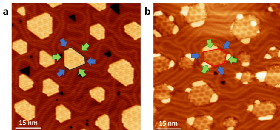
Fig. 5 Edge assignments for (a) FeO/Au(111) ( V_{\text{bias}} = -1.0 V, I = 0.3 nA) and (b) Pd-FeO/Au(111) ( V_{\text{bias}} = -0.8 V, I = 0.3 nA). The blue arrows point to the O-edges while the green arrows point to the Fe-edges. Based on the literature, the short and long edges are O-edges and Fe-edges, respectively. Therefore, the edge assignment is done by first assigning the shortest edge of an island to an O-edge, then identifying the other two alternate O-edges by symmetry, and finally assigning the rest of the edges to Fe edges. The black and red hexagons indicate pointed-top and pointed-bottom configurations of FeO islands.
