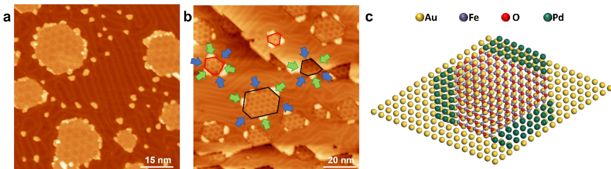
Fig. 4 STM topography of Pd modified FeO/Au(111). (a) As-deposited Pd on FeO/Au(111) ( V_{\text{bias}} = 1.5 V, I = 0.3 nA). (b) Selective growth of Pd on FeO edges following annealing at 550 K ( V_{\text{bias}} = -0.8 V, I = 0.3 nA). The green arrows point to Fe-edges while blue arrows point to O-edges, black and red hexagons indicate pointed-top and pointed-bottom configurations of FeO islands, respectively. (c) Schematic illustration of the atomic structure of Pd-FeO/Au(111).
