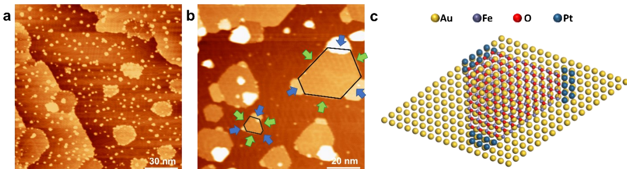
Fig. 6 STM images of Pt modified FeO/Au(111). (a) As-deposited Pt on FeO/Au(111) surfaces ( V_{\text{bias}} = 1.5 V, I = 0.2 nA). (b) Selective growth of Pt on FeO edges following annealing at 550 K ( V_{\text{bias}} = 1.6 V, I = 0.2 nA), the green arrows point to Fe-edges while the blue arrows point to the O-edges. (c) Schematic illustration of the atomic structure of Pt-FeO/Au(111).
