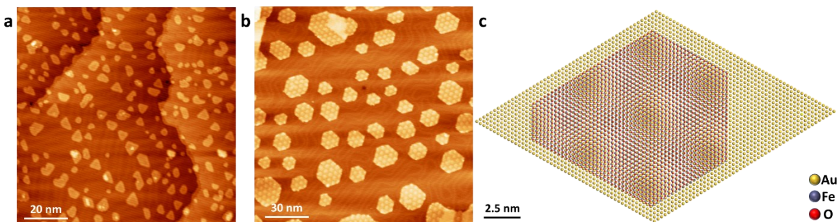
Fig. 1 Growth and structural properties of FeO on Au(111). (a) STM image of sub-monolayer Fe deposited on Au(111) ( V_{\text{bias}} = 1.2 V, I = 0.2 nA). (b) STM topography of FeO islands ( V_{\text{bias}} = 1.5 V, I = 0.5 nA). (c) Schematic illustration of the atomic structure of FeO/Au(111).
