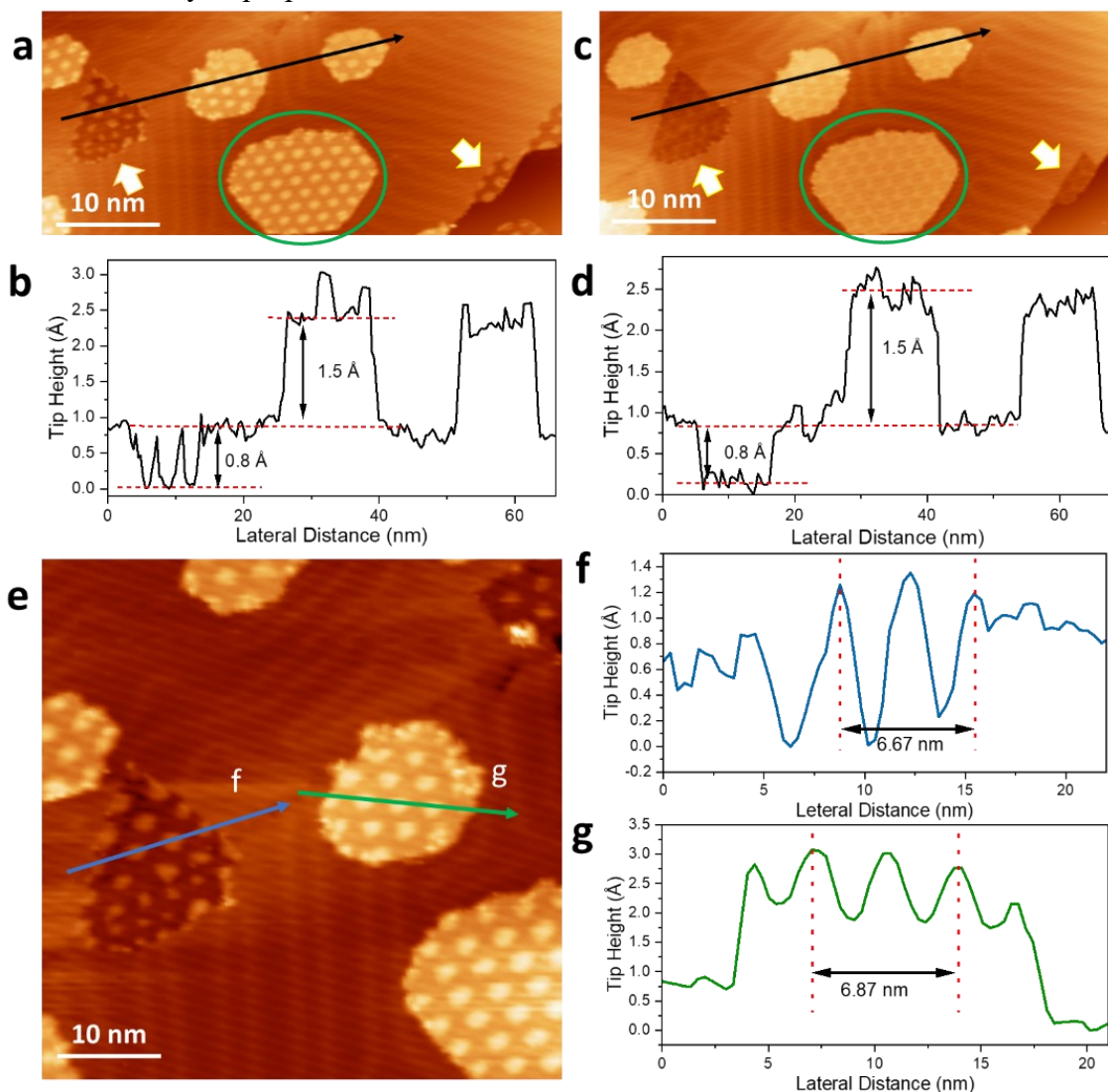
Fig. 3 Bias-dependent STM topography of FeO islands. (a, c) STM images of the same surface obtained under V_{\text{bias}} = 1.7 V (a) and -0.8 V (c) and the same tunneling current I = 0.3 nA. The green circles highlight the same FeO island with different moiré patterns, and the white arrows point to embedded FeO at the center and edge of the terrace. (b, d) Line profiles along the black lines in (a) and (c), respectively. (e) A close look at embedded and supported FeO islands ( V_{\text{bias}} = 1.7 V, I = 0.3 nA). Height profiles of embedded FeO (f) and supported FeO (g), respectively.
