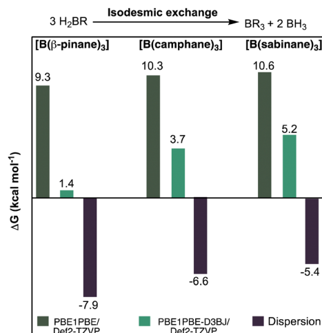
Fig. 4 Calculation results from an isodesmic exchange reaction regarding [B(R)_3] , where R = sabinane, camphane and pinane.
