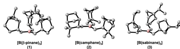
Fig. 3 DFT-optimized structures of complexes 1 – 3 at the PBE1PBE-D3BJ/Def2-TZVP level. Boron shown in pink, carbon in grey and hydrogens are not shown.
