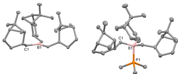
Fig. 5 Molecular structure of complex 4 (thermal ellipsoids at 50% probability), [\text{Me}_3\text{P}-B(\beta\text{-pinane})_3] (right) compared with complex 1 (left). Selected bond lengths (Å) and angles (°) in 4 include B1–P1 = 2.017(12), B1–C1 = 1.640(7), P1–B1–C1 = 107.1(5). Hydrogens are not shown for clarity.
