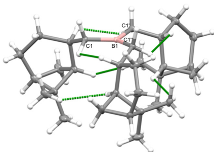
Fig. 2 Molecular structure of compound 1 , [\text{B}(\beta\text{-pinane})_3] . Thermal ellipsoids shown at 50% probability. Inter-ligand \text{H}\cdots\text{H} close contacts are shown in green. Selected bond lengths and angles in 1 include \text{B}1\text{--C}1 = 1.5811(11) Å, \text{C}1'\text{--B}1\text{--C}1 = 119.735(17)^\circ .
