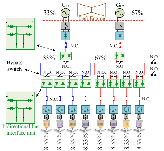
Fig. 9: Current source-based propulsion architecture (half-circuit) [54].
