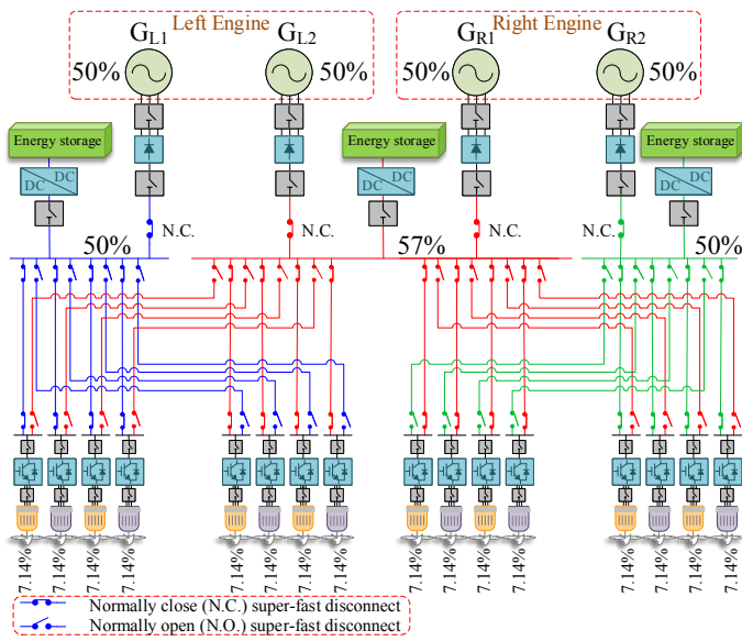
Fig. 8: Voltage source-based three-bus multifeeder architecture using lightweight super-fast disconnects [54].
