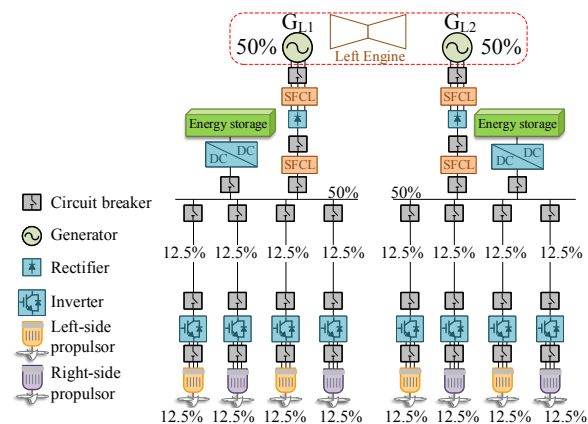
Fig. 4: Baseline propulsion system architecture (half-circuit) [83].
