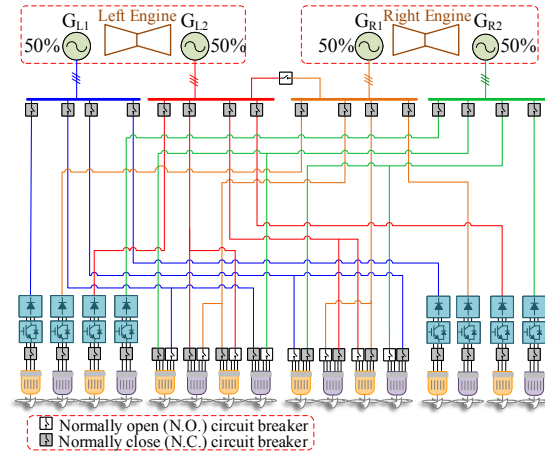
Fig. 11: TeDP topology with an AC-DC architecture. Inboard propulsors are directly connected to the AC buses and outboard ones are being fed from the rectifiers and motor drives [88].
