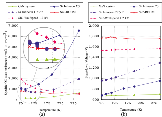
Fig. 25: Comparison of the Si, SiC, and GaN devices (a) specific on-state resistance variation with temperature, and (b) breakdown voltage variation with temperature [168].
