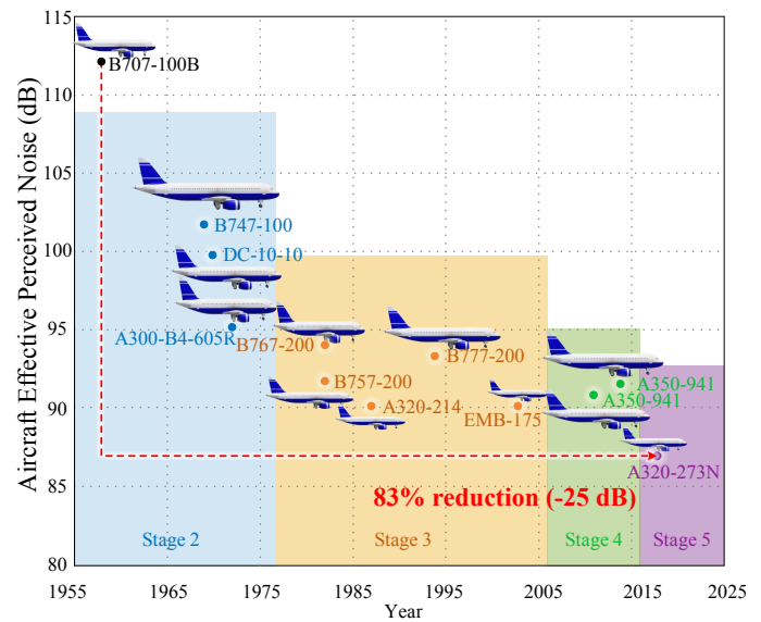
Fig. 1: Effective perceived noise of different aircraft [8].
