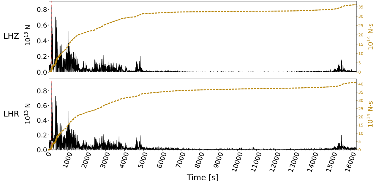
Fig. S12. Vertical reaction force (black) and force impulse (gold) time history from Rayleigh waves. The median stack vertical point-force time histories obtained by deconvolving individual displacement recordings extending for 5000 s (A) and 16,300 s (B) after the source began by corresponding Green's functions for vertical motion (LHZ) and horizontal motion (LHR) of short-arc Rayleigh waves. The uncertainty of the force impulse increases ~10 minutes after the origin time of the M5.8 event (gold dashed line), since the established (two sided) atmospheric oscillatory forces could interfere with the purely positive vertical force.
