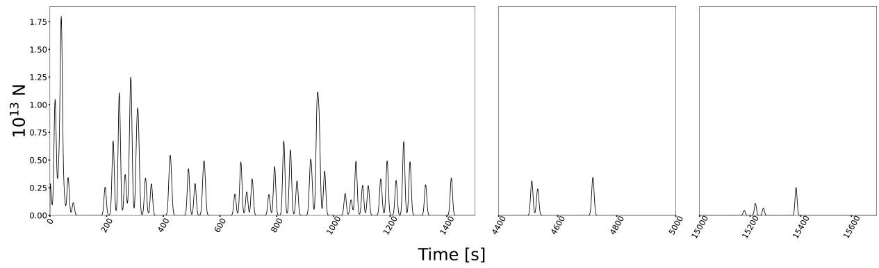
Fig. S7 – Complete time series of the force time history obtained from the simulated annealing waveform inversion. The solution was optimized by fitting the time and amplitude of pulses for windows spanning from 0 - 1500 s, 4400-5000 s and 15000-15700 s.
