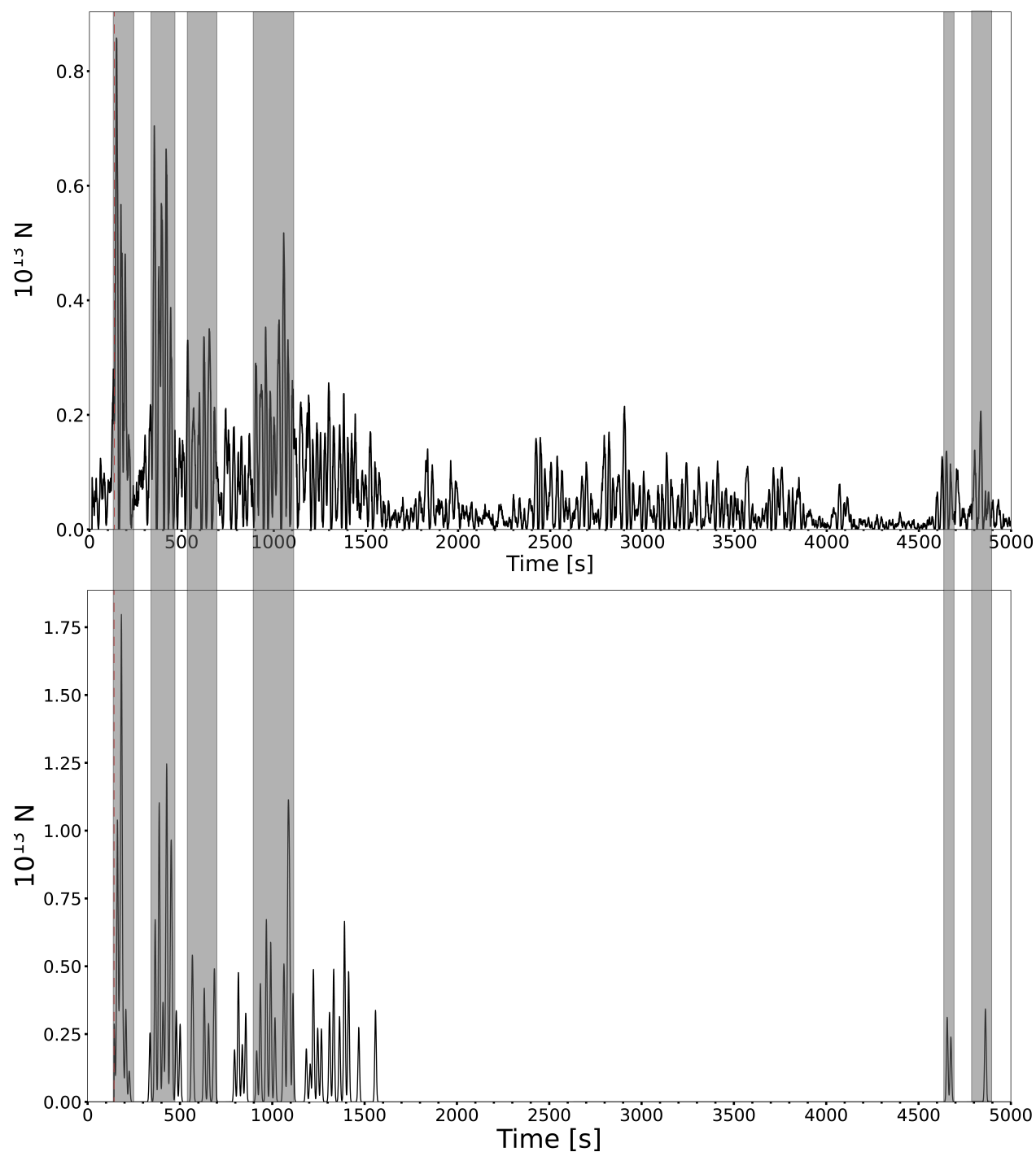
Fig. S11 – Comparison of 5000 s of the force time history calculated from the regional surface waves deconvolution (A) and direct fitting of regional surface waves by the simulated annealing inversion (B).
