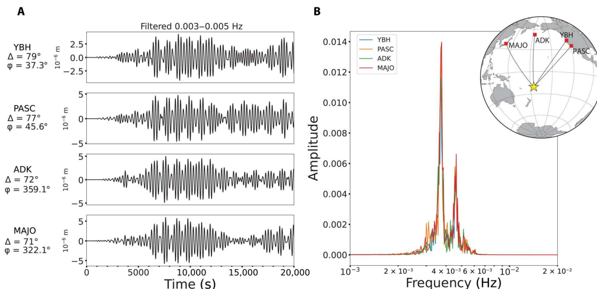
Fig. 7. Long-period Rayleigh waves generated by resonating atmospheric acoustic modes coupled with the solid Earth at the source region. (A) Ground displacements, filtered in the 0.003- to 0.005-Hz passband, recorded at stations ADK, MAJO, PASC, and YBH at varying epicentral distances ( \Delta ) and azimuths from the source ( \phi ). (B) Spectra of the vertical ground motions filtered in the 0.003- to 0.005-Hz passband. Spectral peaks at 3.4 and 4.6 mHz correspond to the frequencies of atmospheric acoustic standing wave modes that couple to the ground to excite Rayleigh waves that spread from the source region.
