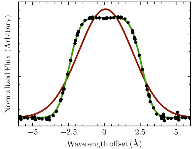
Figure A1. Line-spread function of Keck KCWI with BL grating. We find the LSF of KCWI BL grating to be approximated well by a Gaussian function convolved with a top-hat function, as shown in Equation (A1). To measure the shape of the LSF, we simultaneously fit 31 lines of an FeAr lamp spectrum as described in Appendix A.2. Here, we plot a superposition of the nine most prominent of those lines. Black points mark the flux in the lamp spectrum around each line after normalizing for each line’s amplitude. Our best-fit LSF model (green) has a top-hat function of width \Delta = 5.105 \text{ Å} convolved with a Gaussian function of \sigma = 0.627 \text{ Å} . A single Gaussian function, as is typically assumed, would provide a very poor fit to the KCWI LSF (red).
