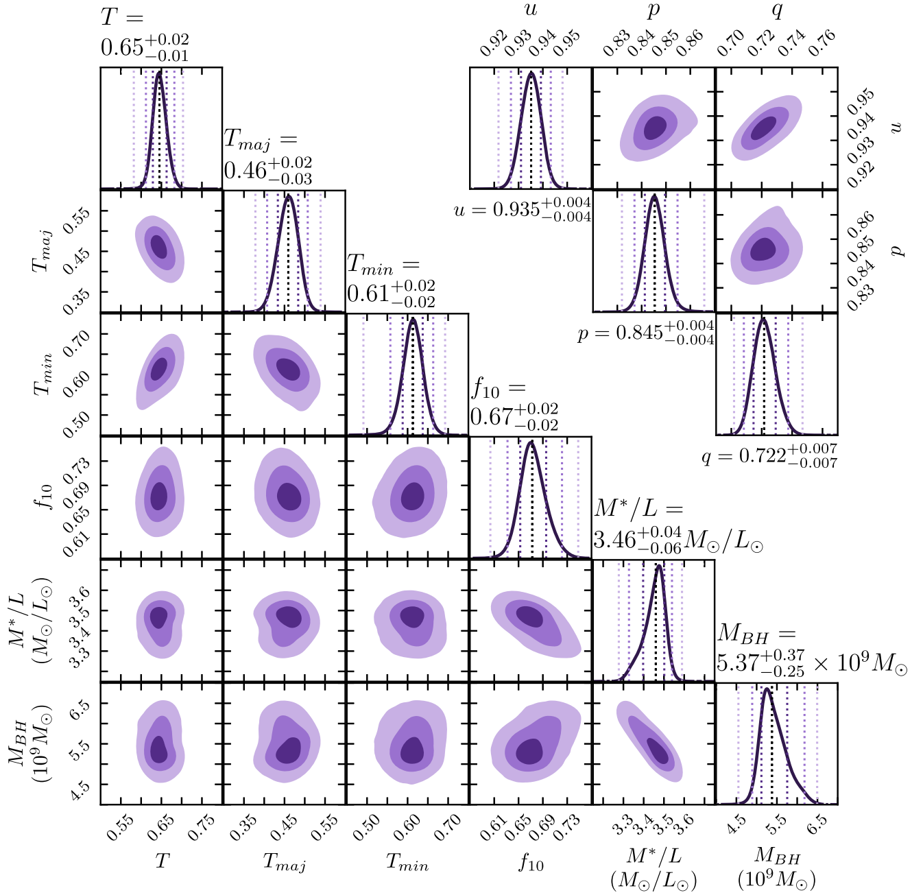
Figure 4. Posterior distributions of six parameters from triaxial Schwarzschild orbit modeling of M87: black hole mass M_{\text{BH}} , outer stellar mass-to-light ratio M^*/L , dark matter fraction enclosed within 10 kpc f_{10} , and shape parameters T , T_{\text{maj}} , and T_{\text{min}} . The posterior distributions of the luminosity-averaged axis ratios u , p , and q are shown in the upper right. The three levels of purple shading bound the 1\sigma , 2\sigma , and 3\sigma regions (68%, 95%, and 99.7% confidence levels, respectively) of the parameters. The vertical lines in each one-dimensional distribution indicate the median and the corresponding three confidence levels.
