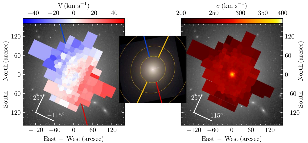
Figure 1. (Left and Right) Stellar kinematic portraits of M87 from Keck KCWI spectra in 461 spatial bins. The line-of-sight velocities (left) and velocity dispersions (right) of stars in M87 are shown over a 250'' by 300'' field of view centered at the galaxy’s nucleus. The systemic velocity of M87 has been removed in the left panel. North is up and east is to the left. The two orthogonal white arrows indicate the orientations of the photometric major axis (PA of -25^\circ ) and minor axis (PA of -115^\circ ), as determined from the mean position angle of the galaxy’s major axis between a radius of 50'' and 250'' in photometric data (Kormendy et al. 2009). The red and blue lines in the left panel mark the measured kinematic axis (PA of -165^\circ ) outward of 70'' (see Figure 2). (Middle) HST composite image of the central 200'' by 200'' FOV of M87, illustrating the misalignment of the photometric major axis (yellow) and kinematic axis (red-blue) beyond 50'' along with sample isophotes of the stellar light distribution (yellow contours).
