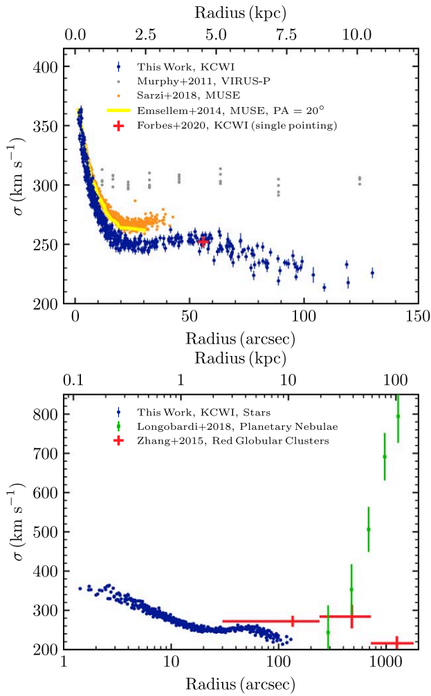
Figure 3. Radial profile of stellar velocity dispersion of M87 in the inner 10 kpc (on a linear scale; top) and out to 100 kpc (on a logarithmic scale; bottom). All 461 KCWI bins are shown (blue) but many overlap. (Top) The KCWI values within 1 kpc agree well with those from MUSE on the Very Large Telescope (Emsellem et al. 2014; Sarzi et al. 2018; yellow and orange, respectively), while the MUSE values are 10–20 km s −1 larger than KCWI between 1 and 3 kpc. At 4.5 kpc, our KCWI measurements match the single data point (red) from an independent KCWI observation (Forbes et al. 2020). The VIRUS-P values (Murphy et al. 2011; gray), which were used in the axisymmetric stellar-dynamical measurement of the M87 black hole (Gebhardt et al. 2011), are 30–50 km s −1 higher than all other measurements. Murphy et al. (2011) noted a similar offset between their values and earlier IFU measurements (Emsellem et al. 2004) in the inner 2 kpc. (Bottom) Red globular clusters have similar \sigma (red) as stars and appear to belong to M87’s stellar halo (Zhang et al. 2015), whereas the intracluster component of planetary nebulae have sharply rising \sigma (Longobardi et al. 2018; green).
