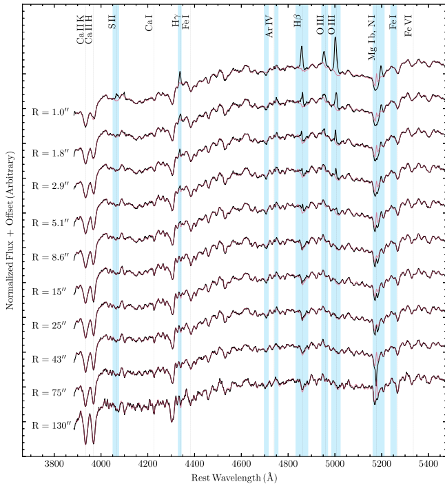
Figure A2. Representative KCWI spectra of M87. Sky-subtracted galaxy spectra (black curves) for ten representative spatial bins located at projected radii from 1'' to 130'' are shown. A total of 461 binned spectra are used in this work. The S/N of these coadded spectra range from about 100 to 200 per Å. The stellar template broadened by the best-fit LOSVD is overlaid (red curves) on each spectrum. Typical fitting residuals are comparable to the line widths. Shaded blue regions indicate masked spectral regions excluded from the analysis. At M87’s redshift, the Mg I b region is contaminated by the 5200 Å [N I] skyline (marked). The central bins exhibit strong AGN emission lines, especially from [O III] (4959 Å and 5007 Å), [S II] (4069 Å and 4076 Å), H \beta (4861 Å), and H \gamma (4330 Å).
