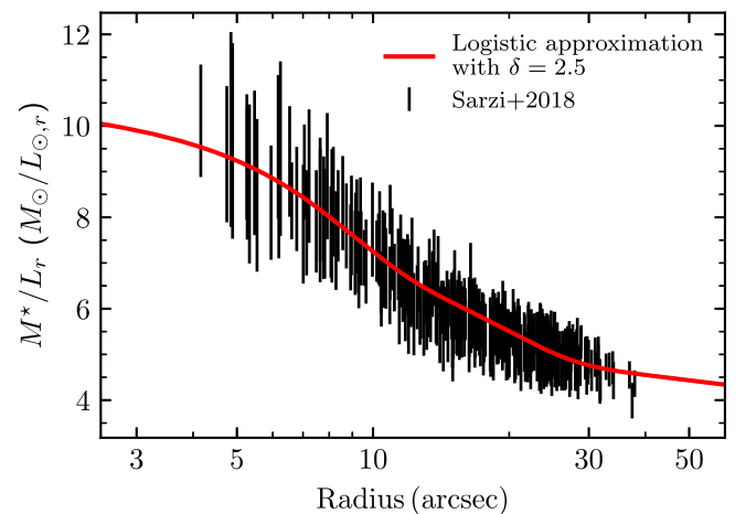
Figure D1. Radial profile of M^*/L ratio used in this work. The logistic approximation (red) used in our modeling, given by Equation (1), is chosen to match the shape of the r -band M^*/L (black) in Figure 11 of Sarzi et al. (2018). The inner M^*/L is \delta = 2.5 times the outer M^*/L ratio, and the transition is centered around 10'' . Our dynamical model prefers an outer V -band M^*/L of 3.46^{+0.04}_{-0.06} M_\odot/L_\odot and inner M^*/L of 8.65^{+0.10}_{-0.15} M_\odot/L_\odot .
