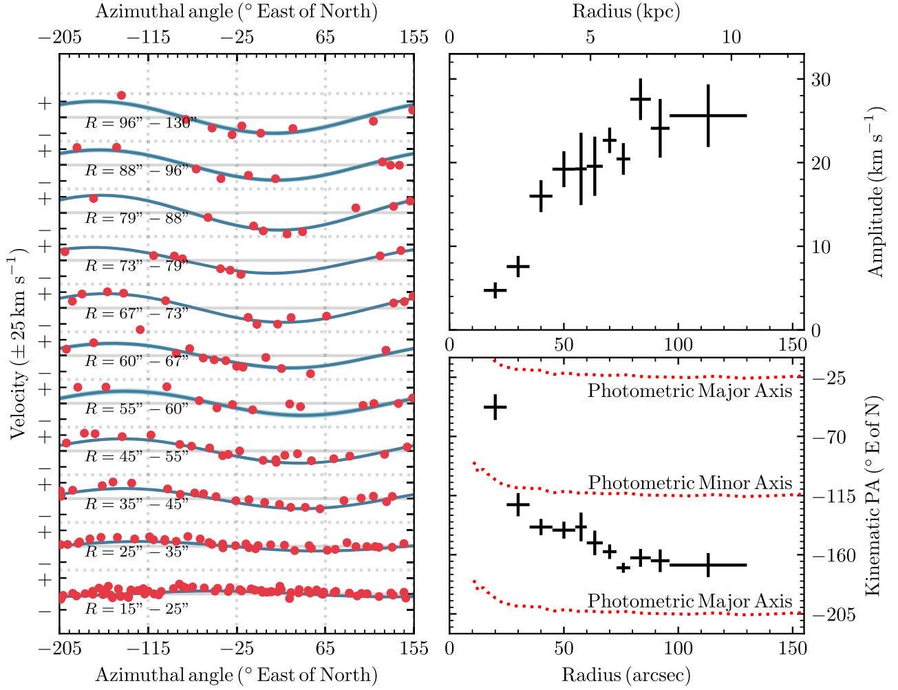
Figure 2. Line-of-sight stellar velocities as a function of projected radius and azimuthal angle on the sky for 11 radial shells spanning R = 15'' – 130'' . The velocities in each shell (red data points) are well fit (blue) by a sinusoidal function of the form V(R, \Theta) = V_1(R) \cos[\Theta - \Theta_0(R)] . (Upper right) The amplitude of rotation, V_1(R) , increases with radius and reaches 25 \text{ km s}^{-1} around 6 kpc. (Lower right) The phase of the velocity function, \Theta_0 , measures the orientation of the kinematic axis and varies significantly with radius. It plateaus to -165^\circ beyond 6 kpc, indicating a 40^\circ misalignment between the kinematic axis and the photometric major axis (red dashed curves; Kormendy et al. 2009) in M87.
