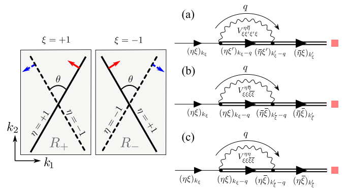
FIG. 2. Left: Configurations of the FAs where solid and dashed lines denote the states on the two surfaces ( \eta = \pm 1 ). \xi = \pm 1 are two FAs on the same surface, at momentum region R_\xi . Directions of dispersions are marked by arrows. Pairs of FAs with \xi\eta = \pm 1 are nested with momentum \vec{Q} , which disperse in opposite directions. Right: Self-energy diagrams which describe spontaneously broken symmetries. k_\xi , q represent four vectors, with momenta \vec{k}_\xi \in R_\xi . (a), (b), and (c) gives rise to self-energies for D-ex, FFLO-ex, and CDW orders, respectively. ■ stands for any of (\eta, \xi) .
