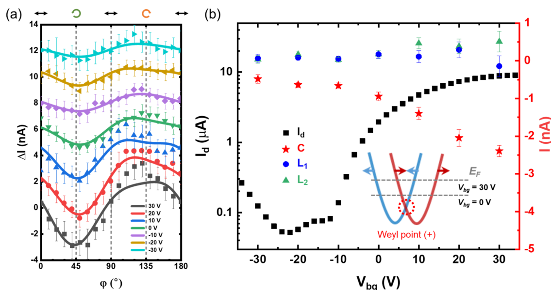
Figure 3. Gate-tunable circular photogalvanic effect in 2D Te. (a) The polarization-dependent photocurrent \Delta I as a function of the quarter-wave plate angle \phi at different back gate voltages. (b) Output characteristic (black) of a 2D Te field-effect transistor. Fit results calculated from (a): C (red), L_1 (blue), and L_2 (green) as a function of the back gate voltage V_{bg} . Inset in (b): the band structure of 2D Te. The back-gate voltage tunes the Fermi level indicated by the dashed line.
