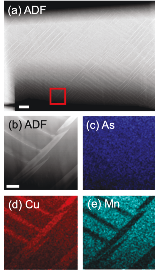
FIG. 4. For the Cu-rich \text{Cu}_{1.18}\text{Mn}_{0.82}\text{As} sample, STEM micrographs of a FIB liftout reveal a tweed-like pattern in ADF imaging. The boxed area is shown in panels [(b)–(e)] for ADF, As, Cu, and Mn EDS maps. Scale bars are 500 nm in (a) and 100 nm in [(b)–(e)].
