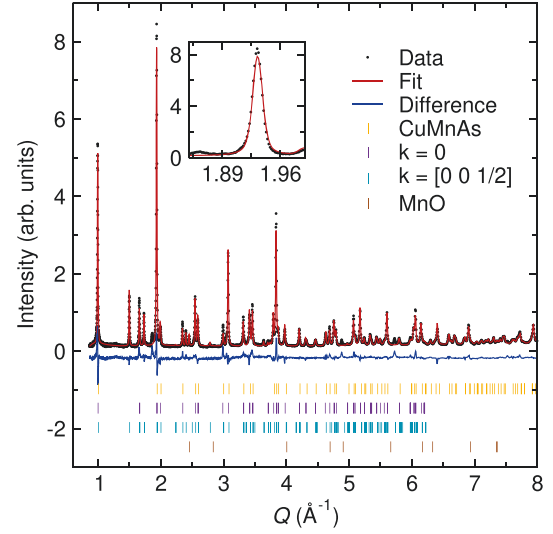
FIG. 6. Rietveld fit to the POWGEN NPD data of the Mn-rich \text{Cu}_{0.64}\text{Mn}_{1.36}\text{As} sample at 300 K. The inset figure shows that unlike at 500 K, the 101 peaks does not show splitting, so there is no evidence for phase separation from structural peaks alone. However, magnetic peaks are present for both the k = 0 (CuMnAs-like) and k = 00\frac{1}{2} ( \text{Mn}_2\text{As} -like) magnetic ordering.
