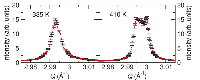
FIG. 2. The 003 synchrotron XRD peak is shown at 335 K and 410 K for the same \text{Cu}_{1.18}\text{Mn}_{0.82}\text{As} sample as the temperature map in Fig. 3(a). At least three peaks are apparent at 410 K.
