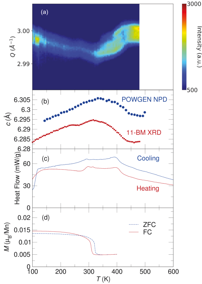
FIG. 3. For the Cu-rich sample \text{Cu}_{1.18}\text{Mn}_{0.82}\text{As} , the in-situ synchrotron XRD measurements (collected on heating) have sufficient resolution to observe splitting in the higher-order 003 peak, which is shown in (a). (b) Shows the change in c lattice parameter across temperature as determined from a single-peak fit to the 001 reflections in synchrotron XRD and POWGEN NPD measurements. The DSC heating (inverted) and cooling curves are shown in (c) and the field cooling and zero-field cooling curves are shown in (d). More than two phases are present in the intermediate temperature range from 300 to 400 K.
