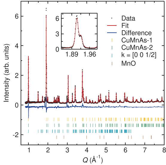
FIG. 5. Rietveld fit to the POWGEN NPD data of the Mn-rich sample \text{Cu}_{0.64}\text{Mn}_{1.36}\text{As} at 500 K shows the presence of two closely-related tetragonal CuMnAs phases. The inset shows the split 101 peak that indicates a clear phase separation. One of the phases displays a \text{Mn}_2\text{As} -like k = [00\frac{1}{2}] magnetic peak (as opposed to the k = 0 magnetic structure of near-stoichiometric CuMnAs). The peak at Q = 1.9 \text{ \AA}^{-1} could not be assigned, and appeared irreversibly upon initial heating.
