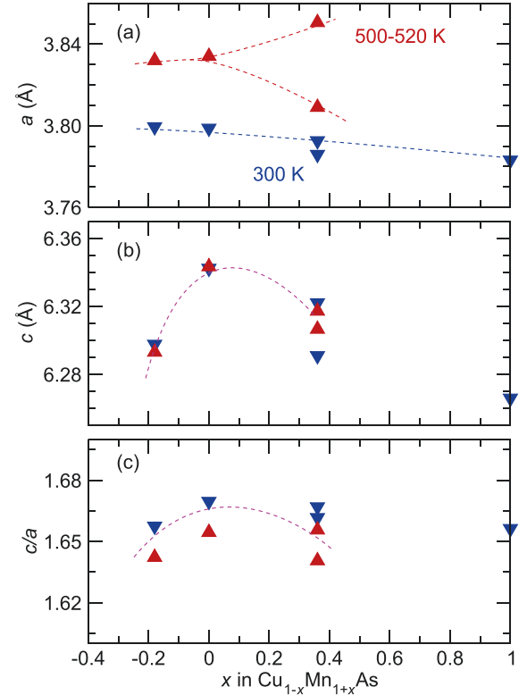
FIG. 8. The lattice parameters across various compositions obtained using NPD refinements to T = 300 and 500 \text{ K} data. T = 300 \text{ K} data for the Cu-excess and the near-stoichiometric sample are taken from x-ray diffraction measurements. Compositions are nominal. Values for \text{Mn}_2\text{As} are from Nuss et al. [47]. It is clear in (a) that an opposing trend in composition versus a appears above and below T_N , but this trend must be broken as x increases toward \text{Mn}_2\text{As} , and the \text{Cu}_{0.64}\text{Mn}_{1.36}\text{As} composition has separated into two phases. In (b), the relative splittings in c are less variable with temperature but exhibit a maximum around the equiatomic CuMnAs composition. The c/a ratios in c are dominated by the trends in c . The dashed lines are used as a guide for observing trends.
