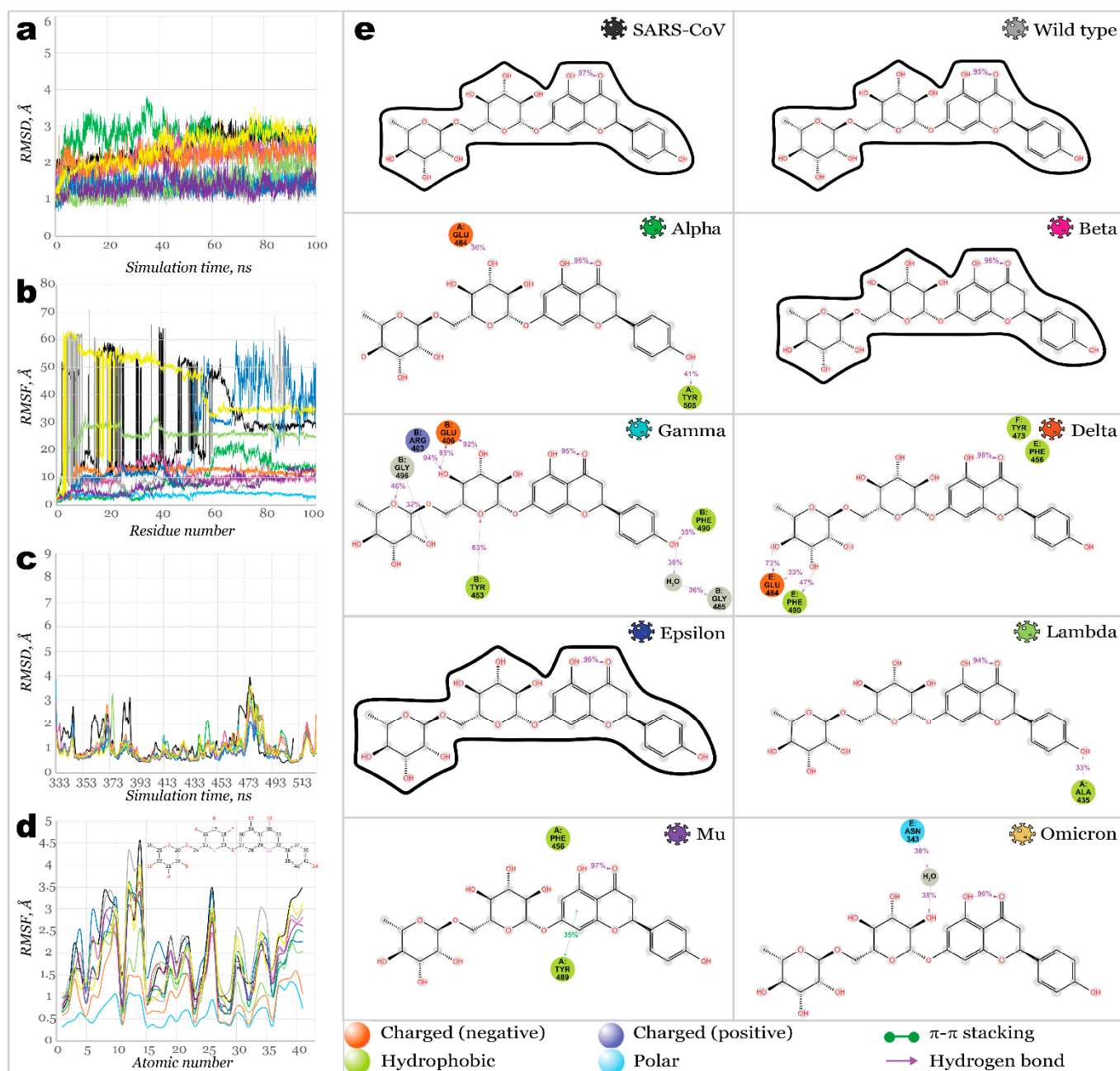
Figure 8. 100 ns MD simulations results for RBD38 (narirutin) complexes: (a)—RMSD of protein's C_{\alpha} ; (b)—RMSF of protein structures; (c)—RMSD of ligand fit on protein; (d)—RMSF of ligand's structures; (e)—2D interactions diagram for narirutin and RBDs.
