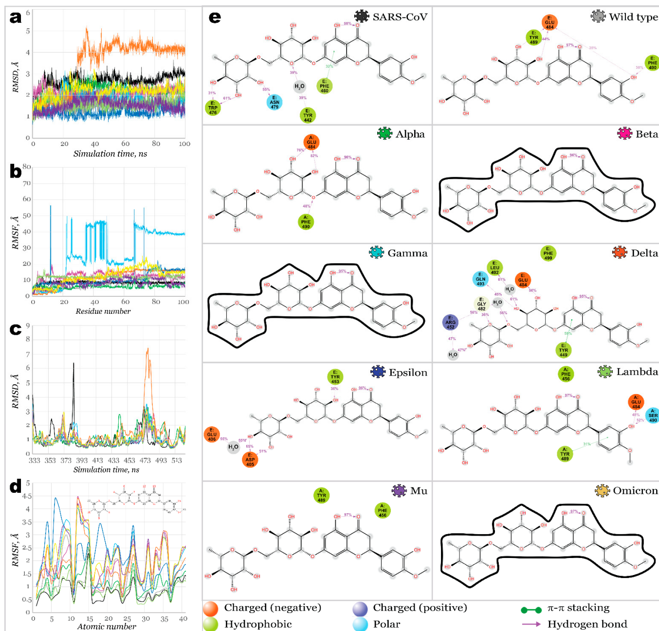
Figure 7. 100 ns MD simulations results for RBD28 (hesperidin) complexes: (a)—RMSD of protein's C_{\alpha} ; (b)—RMSF of protein structures; (c)—RMSD of ligand fit on protein; (d)—RMSF of ligand's structures; (e)—2D interactions diagram for hesperidin and RBDs.
