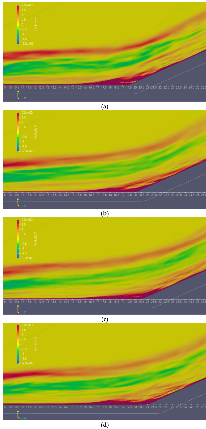
Figure 9. In time-average view, the vorticity distribution on the streamwise central plane, (a) case 1, (b) case 2, (c) case 3, (d) case 4.
