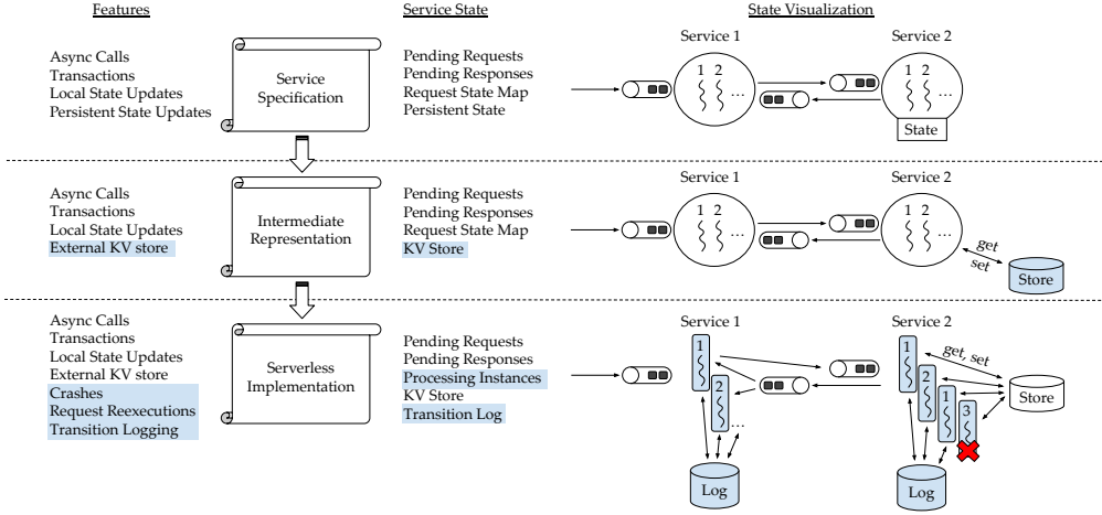
Fig. 2. μ2sls overview: The three abstraction layers that are defined in the framework. The components highlighted in light blue are the ones that differ from the layer above.
