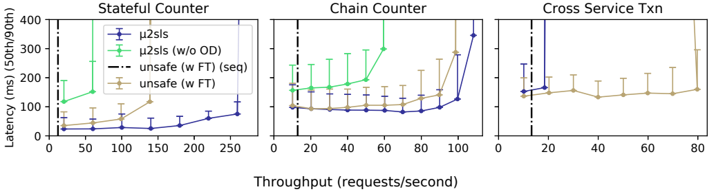
Fig. 11. Transactions Overhead (Q2): Comparison of \mu 2sls , \mu 2sls (w/o OD) (no optimized dictionary wrapper), and unsafe (w/ FT) (no transactional guarantees). unsafe (w/ FT) (seq) shows the throughput of the implementation without transactional guarantees when executed with sequential load.
