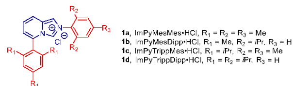
Figure 2. Structures of imidazo[1,5-a]pyridin-3-ylidene ligands used in this study.
