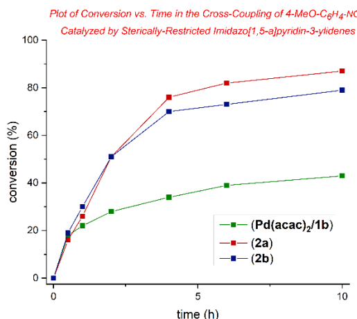
Figure 3. Kinetic profile of the Suzuki-Miyaura cross-coupling of 4-MeO-C 6 H 4 -NO 2 with phenylboronic acid catalyzed by Pd(acac) 2 /1b, 2a and 2b at 130 °C.
