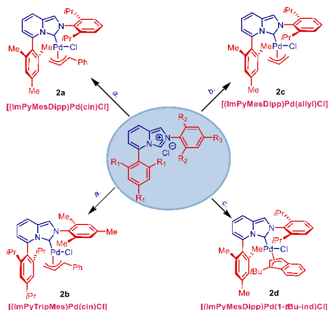
Scheme 1. Synthesis of Pd(II)–NHC Complexes a
