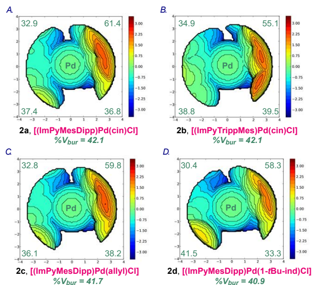
Figure 5. Topographical steric maps of [(ImPyMesDipp)Pd(cin)Cl] ( 2a ) (A), [(ImPyTrippMes)Pd(cin)Cl] ( 2b ) (B), [(ImPyMesDipp)Pd(allyl)Cl] ( 2c ) (C), [(ImPyMesDipp)Pd(1- t Bu-ind)Cl] ( 2d ) (D) showing % V_{bur} per quadrant.
