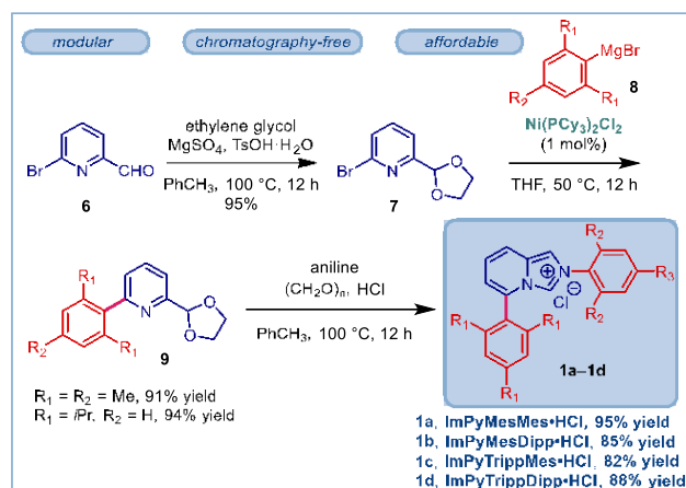
Scheme 2. Modular and Chromatography-Free Synthesis of ImPy Ligands via Ni-Catalyzed Kumada Cross-Coupling
