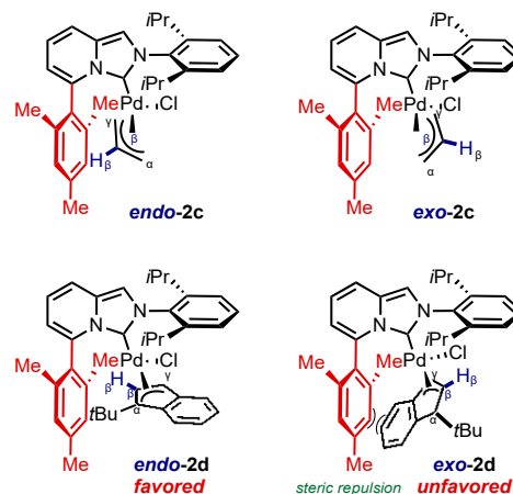
Chart 1. Endo and exo isomers of Pd(II)–NHC Complexes 2a–2d
