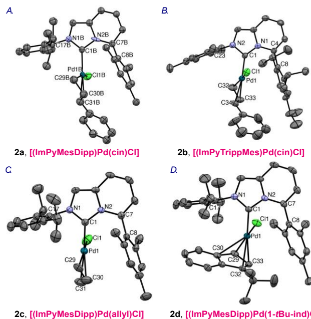
Figure 4. X-ray structure of complex 2a (A), 2b (B), 2c (C), 2d (D). Hydrogen atoms have been omitted for clarity. See SI for selected bond lengths and angles. CCDC 2174493 ( 2a ); CCDC 2174494 ( 2b ); CCDC 2174495 ( 2c ); CCDC 2174496 ( 2d ).
