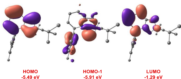
Figure 6. HOMO ( \pi -donating orbital), HOMO-1 ( \sigma -donating orbital) and LUMO ( \pi -accepting orbital) of imidazo[1,5- a ]pyridin-3-ylidene 1b . B3LYP 6-311++g(d,p) level. See SI for details.
