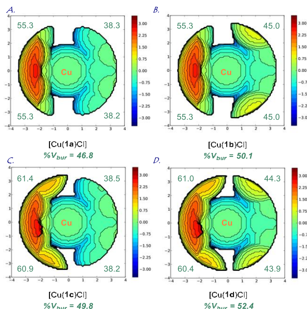
Figure 7. (A–D) Topographical steric maps of linear imidazo[1,5- a ]pyridin-3-ylidenes [Cu(NHC)Cl] ( 1a–1d ) showing % V bur per quadrant. B3LYP 6-311++g(d,p) level. See SI for details.
