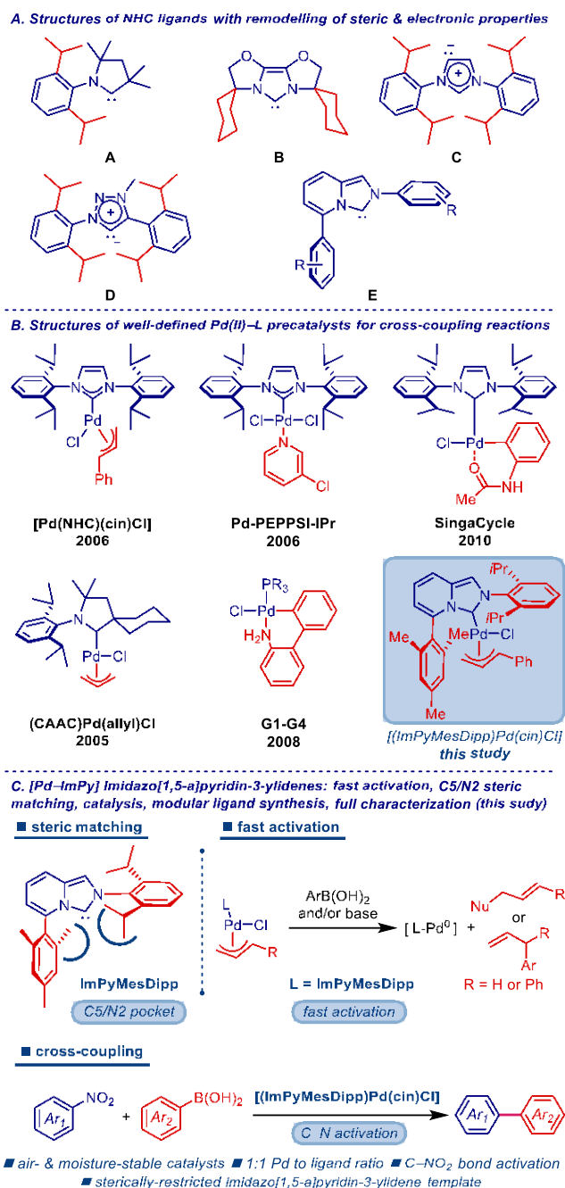
Figure 1. (A) Electronic and structural remodelling of NHC ligands. (B) State-of-the art Pd(II) precatalysts in cross-coupling reactions. (C) Pd(II)-ImPy and steric-matching of [(ImPyMesDipp)Pd(cin)Cl] as air-stable, fast-activating, sterically-restricted Pd(II)-NHC precatalysts.
