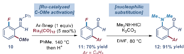
Scheme 4. Sequential Ru(0)-Catalyzed C–OMe Activation/Nucleophilic Aromatic Substitution.
