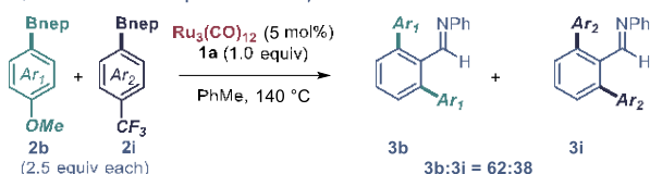
Scheme 6. Mechanistic Studies.
