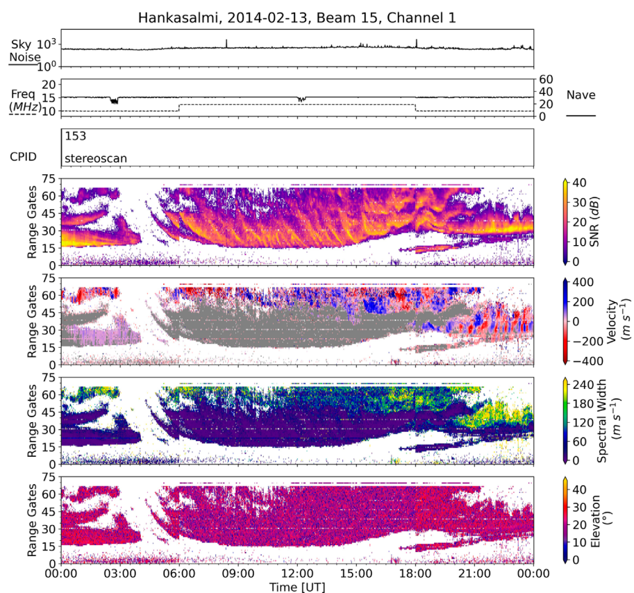
FIGURE 4 Summary plot for beam 15 of the Hankasalmi SuperDARN radar showing power, velocity, spectral width and elevation angle parameters on 13 February 2014.
