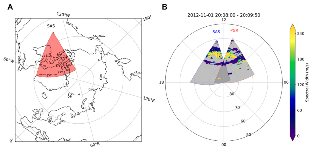
FIGURE 5 FOV plot (left) for the Saskatoon radar and fan plot (right) for the Saskatoon and Prince George radars at 20:08 UT on 1 November 2012.
