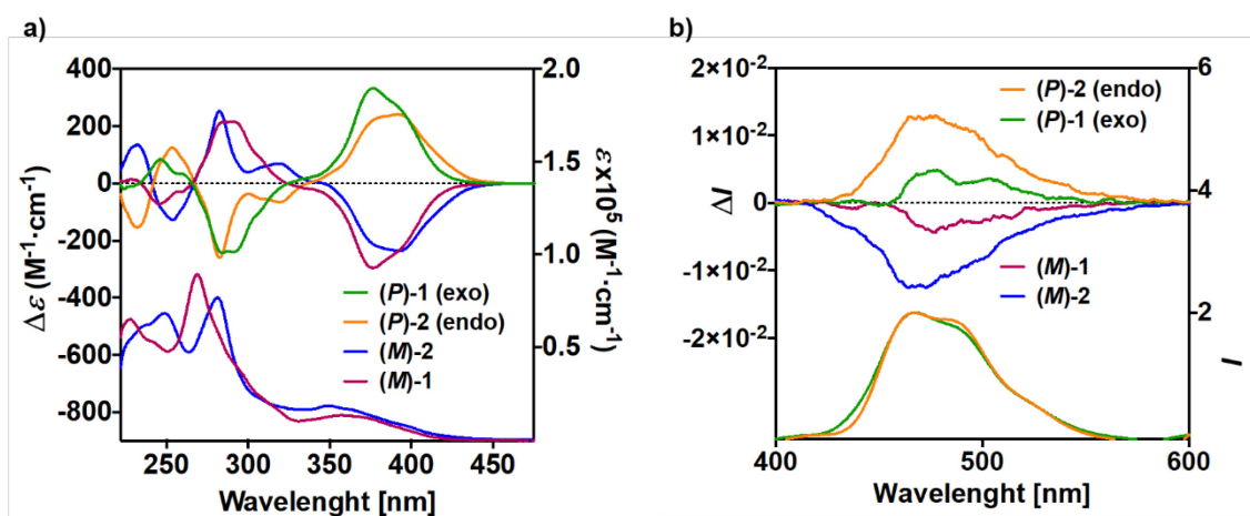
Figure 2. a) Experimental UV-vis (bottom) and ECD (top) spectra and b) fluorescence (bottom) and CPL (top) spectra of ( P ) and ( M ) enantiomers of 1 and 2 (CH 2 Cl 2 , C \sim 10^{-5} M).
