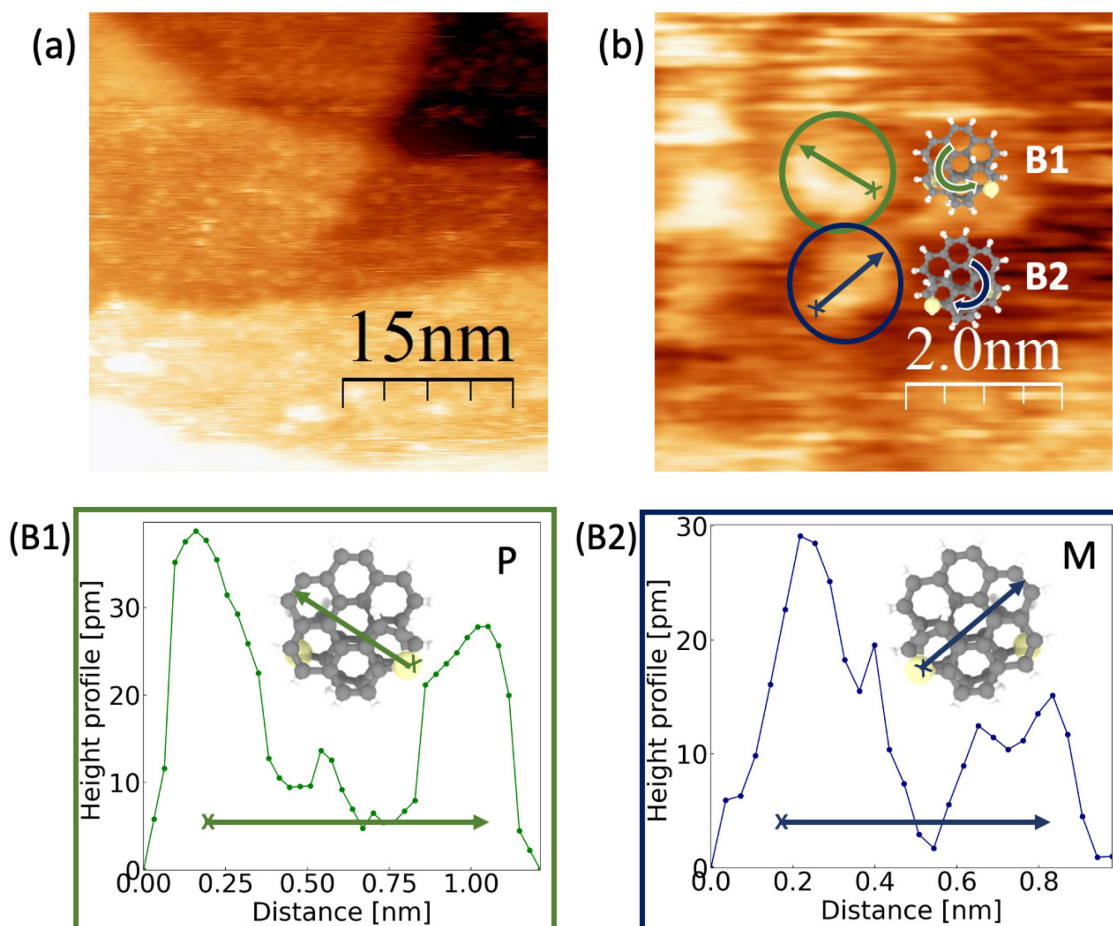
Figure 9. Panel (a) shows a topographic image of exo -dithia[9]helicene acquired using V_{\text{bias}} = 0.5 V and I_t = 0.1 \cdot 10^{-9} A. (b) Zoomed in image of two enantiomer with chirality P in green and M , in blue, and the corresponding height profiles for each enantiomer (B1 for P and B2 for M ). The set parameters were V_{\text{bias}} = 0.4 V and I_t = 0.1 \cdot 10^{-9} A.
