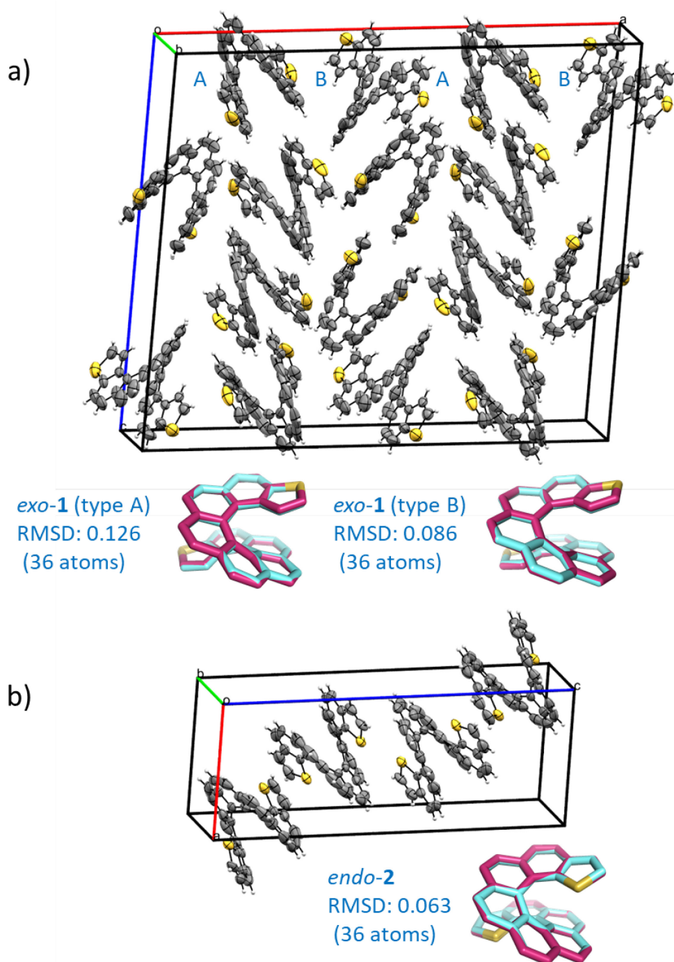
Figure 1. a) Crystal structure of the racemate exo -dithia[9]helicene ( 1 ): Monoclinic unit cell, space group C2/c, a = 33.075(4) , b = 9.8984(11) , c = 28.178(3) (Å); \alpha = 90 , \beta = 94.890(2) , \gamma = 90^\circ ; Z = 16 ; CCDC number 2184340;. The experimental structures of both molecular types found in the unit cell (A and B, reported in cyan) are overlapped with the calculated CAM-B3LYP/def2-SV(P) structures (in magenta) and shown below the unit cell; b) Crystal structure of the racemate endo -dithia[9]helicene- 2 : Monoclinic unit cell, space group P2 1 /n, a = 9.712(2) , b = 9.709(3) , c = 25.072(6) (Å); \alpha = 90 , \beta = 94.401(7) , \gamma = 90^\circ ; Z = 4 ; CCDC number 2184341. The experimental and calculated (CAM-B3LYP/def2-SV(P)) structures, reported in cyan and magenta respectively, are overlapped and shown below the unit cell. The root mean square deviation (RMSD, in Å) is calculated considering only the heavy atoms of an isolated dithia[9]helicene of ( M )
