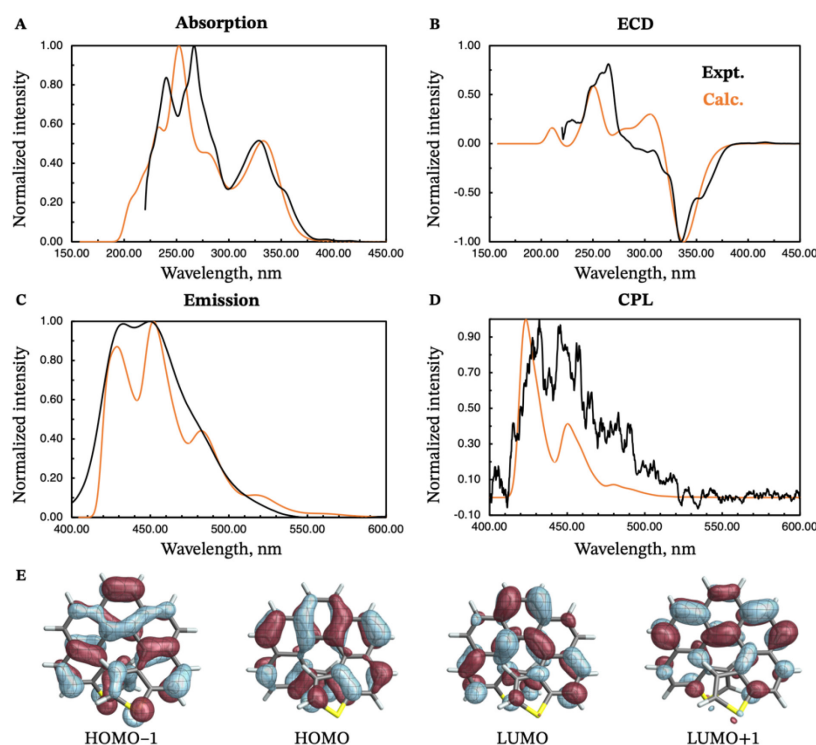
Figure 7 Experimental (black curves) and calculated (orange curves) absorption (panel A), ECD (panel B), emission (panel C) and CPL (panel D) spectra of ( M )- exo -dithia[7]helicene 10 . Isosurfaces ( \pm 0.03 au) for the most relevant frontier molecular orbitals (HOMO–1, HOMO, LUMO, and LUMO+1) are shown in panel E. The calculated energies were shifted by -0.40 eV prior to conversion to wavelengths.
