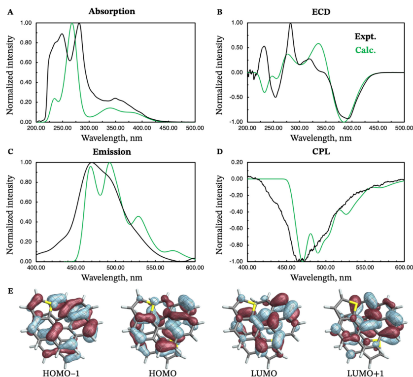
Figure 6 Experimental (black curves) and calculated (green curves) absorption (panel A), ECD (panel B), emission (panel C) and CPL (panel D) spectra of ( M )- endo -dithia[9]helicene 2 . Isosurfaces ( \pm 0.03 au) for the most relevant frontier molecular orbitals (HOMO–1, HOMO, LUMO, and LUMO+1) are shown in panel E. The calculated energies were shifted by -0.40 eV prior to conversion to wavelengths.
