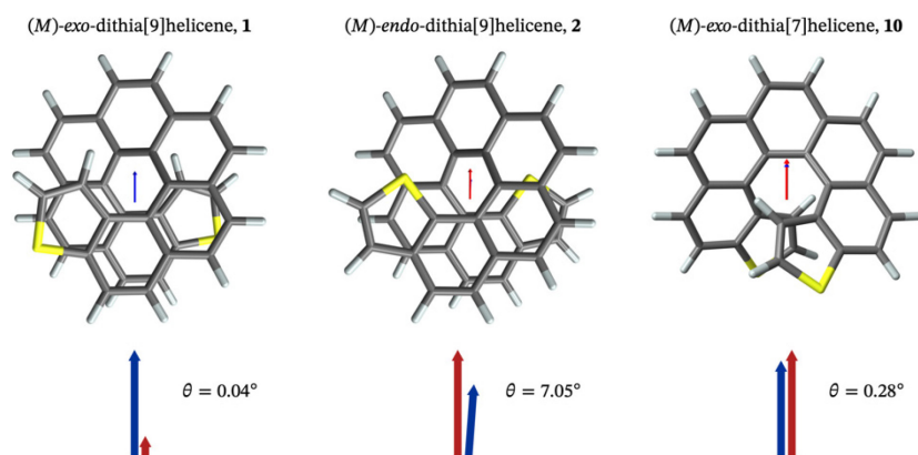
Figure 4 Electric ( \vec{\mu}_e , red arrows) and magnetic ( \text{Im}[\vec{\mu}_m^*] , blue arrows) transition dipole moments—arbitrarily scaled relative to the images of the excited state ( S_1 ) geometry—for the S_1 – S_0 transition for the ( M ) isomers of exo -dithia[9]helicene (panel A ), of endo -dithia[9]helicene (panel B ), and of exo -dithia[7]helicene (panel C ) obtained from TD-DFT calculations. For clarity, the electric and magnetic dipole moments are also shown, magnified, below the calculated geometries. The angle \theta (in degrees) between the two vectors is shown as well. The transition moment vectors are collinear with the C_2 axis of the three compounds.
