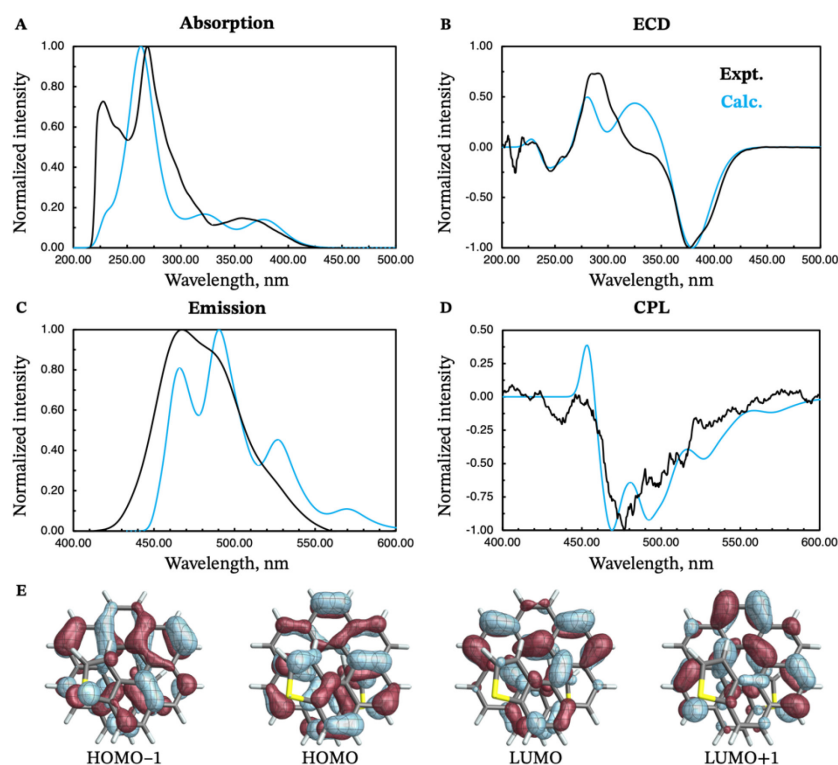
Figure 5 Experimental (black curves) and calculated (blue curves) absorption (panel A), ECD (panel B), emission (panel C) and CPL (panel D) spectra of ( M )- exo -dithia[9]helicene 1 . Isosurfaces ( \pm 0.03 au) for the most relevant frontier molecular orbitals (HOMO-1, HOMO, LUMO, and LUMO+1) are shown in panel E. The calculated energies were shifted by -0.40 eV prior to conversion to wavelengths.
