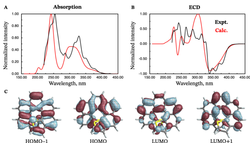
Figure 8 Experimental (black curves) and calculated (red curves) absorption (panel A) and ECD (panel B) spectra of ( M )- endo -dithia[7]helicene 11 . Isosurfaces ( \pm 0.03 au) for the most relevant frontier molecular orbitals (HOMO–1, HOMO, LUMO, and LUMO+1) are shown in panel C. The calculated energies were shifted by -0.40 eV prior to conversion to wavelengths.
