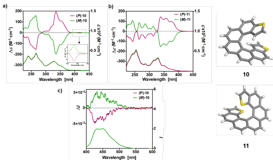
Figure 3. The experimental UV-vis (bottom) and ECD (top) spectra of the ( P ) and ( M ) isomers of 10 and 11 ( \text{CH}_2\text{Cl}_2 , C \sim 10^{-5} M) are shown in panels a) and b), respectively. The inset in a) shows the magnified ECD of ( P ) and ( M )- 10 in the 400-450 nm region. The fluorescence (bottom) and CPL (top) spectra of ( P ) and ( M )- 10 are shown in panel c).
